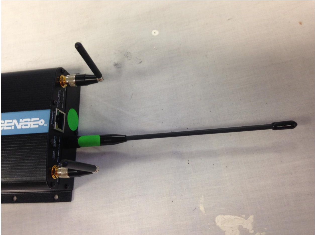
Figure 2. Antenna on EUT
