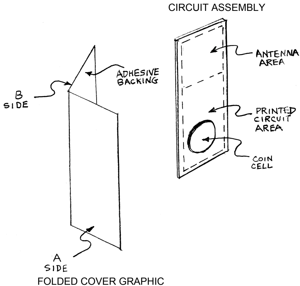
FIGURE 2. PLACEMENT OF COVER GRAPHIC
