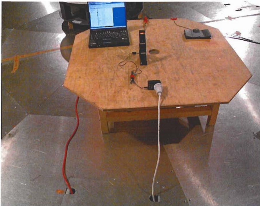
Fig. 6.3.1: Basic set-up for conducted emission test from power ports
