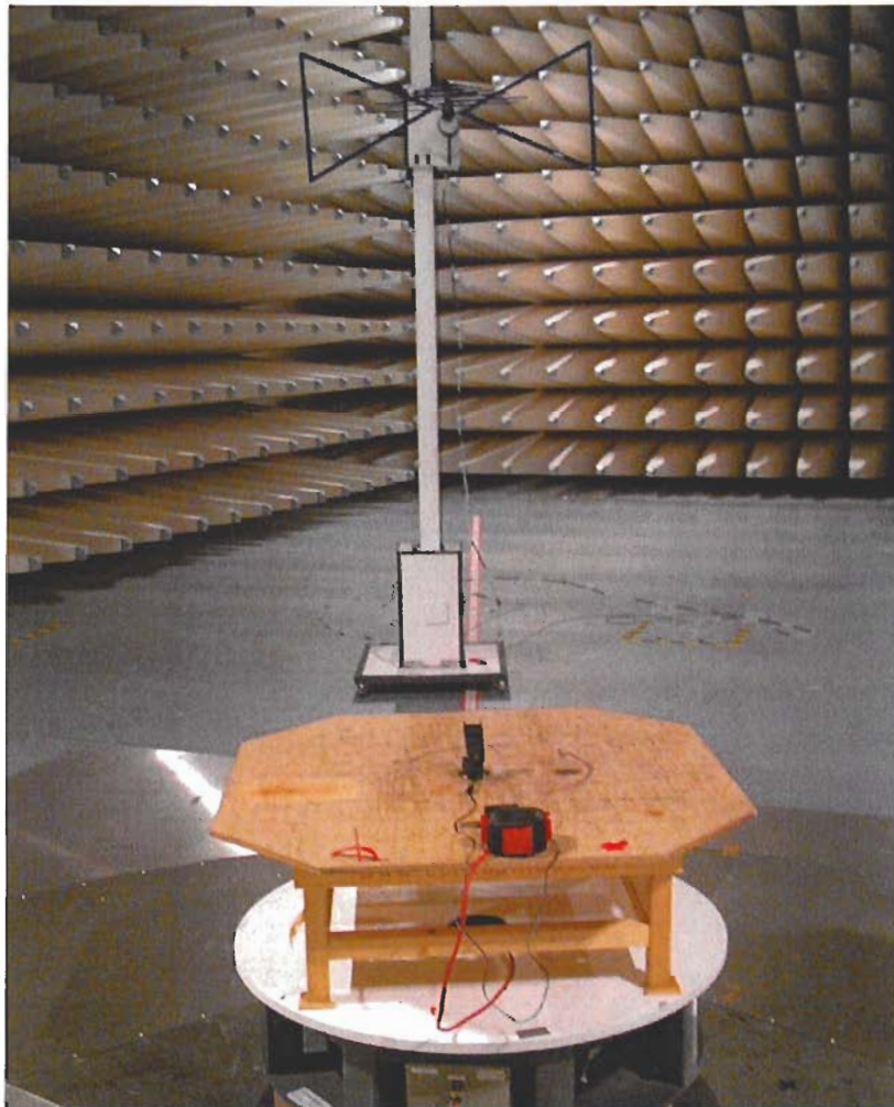
Fig. 5.2.1: Basic set-up for radiated emission; 30 MHz - 1 GHz
