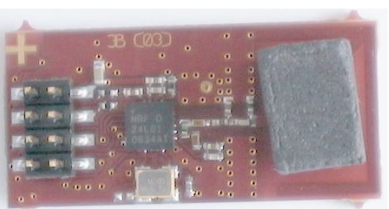
Digita CordEx Station wireless PCB top side with distance piece
