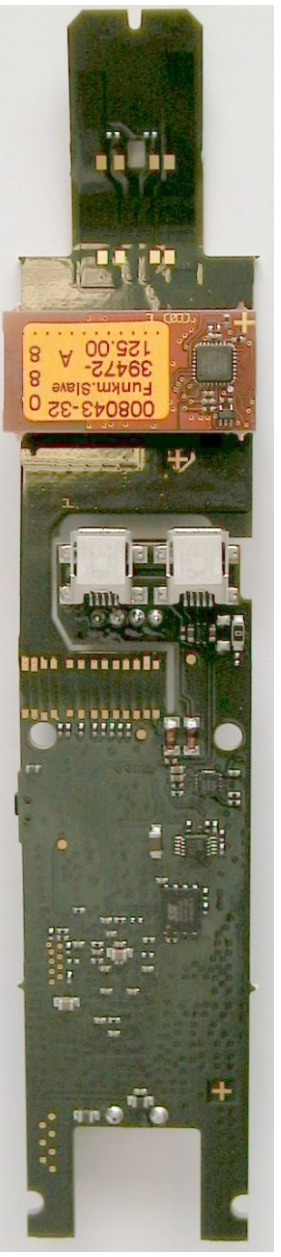
Digta CordEx Station PCB bottom side with wireless-modul
