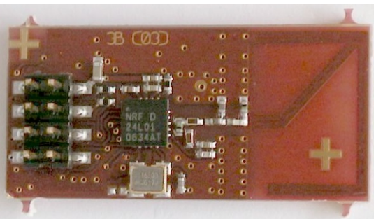
Digita CordEx Station wireless PCB top side
