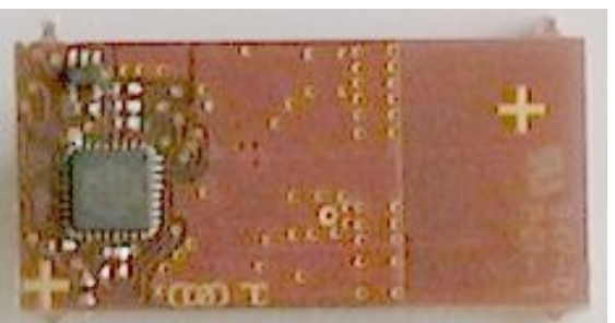
Digita CordEx Station wireless PCB bottom side
