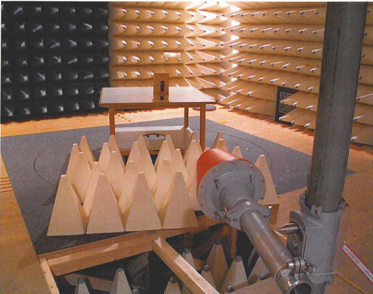
Fig. 5.2.2: Basic set-up for radiated emission test above 1 GHz distance 3m
