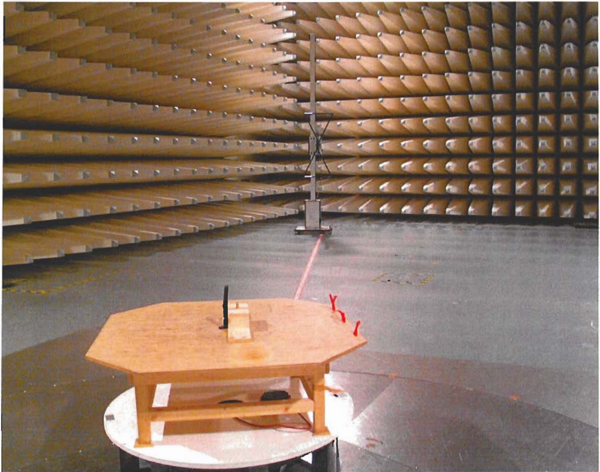
Fig. 5.2.1: Basic set-up for radiated emission; 30 MHz - 1 GHz distance 10m
