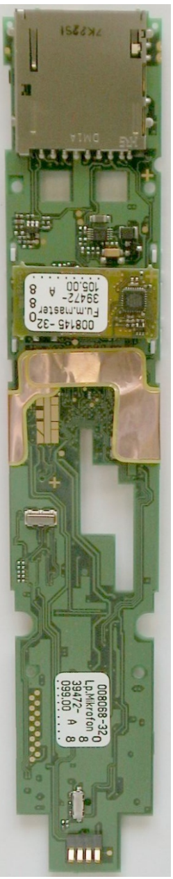
Digta CordEx Microphone PCB bottem side with wireless-modul and shielding
