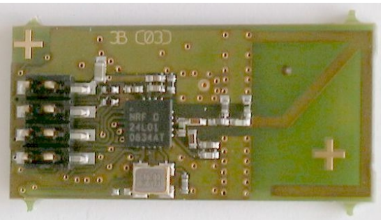
Digita CordEx Microphone wireless PCB top side
