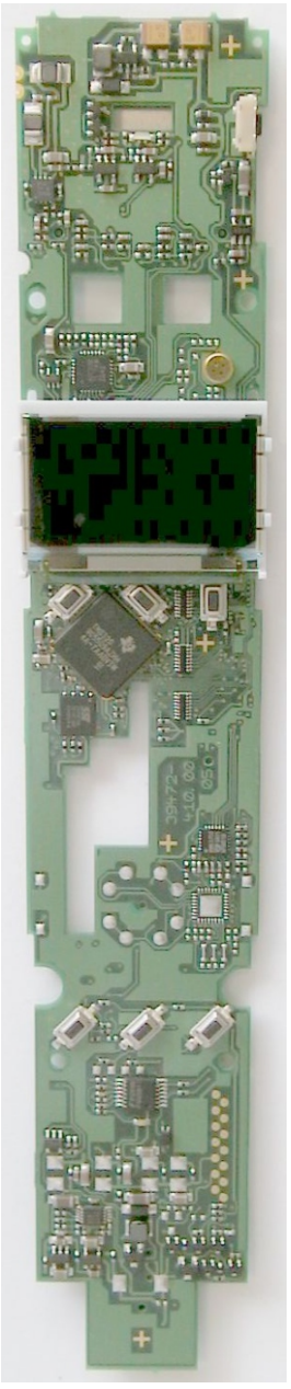
Digita CordEx Microphone PCB top side with display
