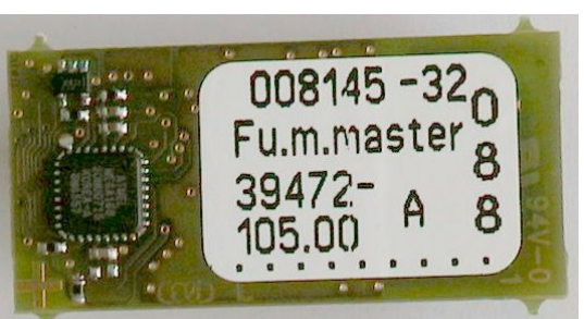
Digita CordEx Microphone wireless PCB bottom side with Label
