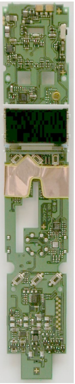
Digita CordEx Microphone PCB top side with display and shielding
