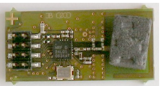
Digita CordEx Microphone wireless PCB top side with distance piece
