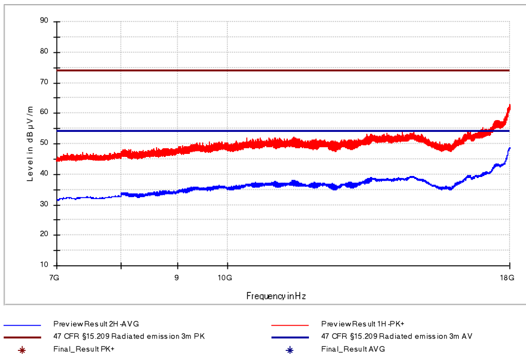
Figure 14: Chart of emissions test from 7 GHz to 18 GHz without tag in position Z and antenna polarization H
