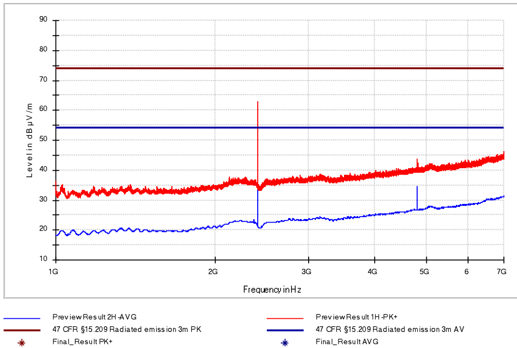
Figure 13: Chart of emissions test from 1 GHz to 7 GHz without tag in position Z and antenna polarization H (with 2.4 GHz notch filter)
