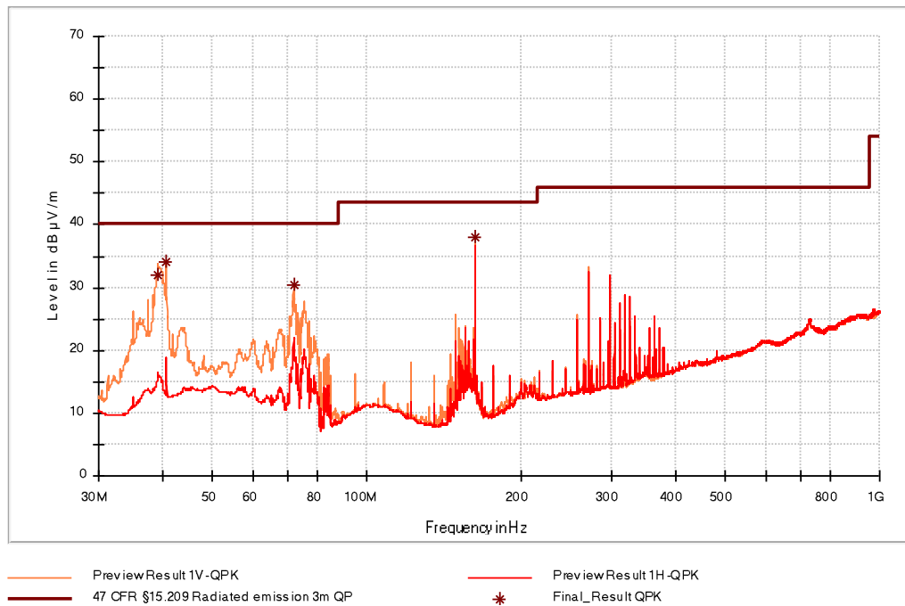
Figure 12: Chart of emissions test from 30 MHz to 1 GHz with tag in position Z
