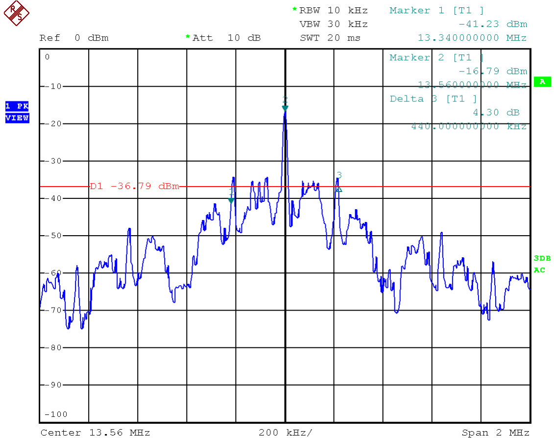
Figure 8: Chart of 20 dB bandwidth
