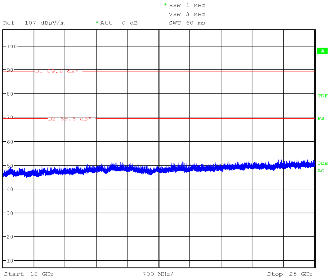
Figure 15: Chart of emissions test from 18 GHz to 25 GHz without tag
