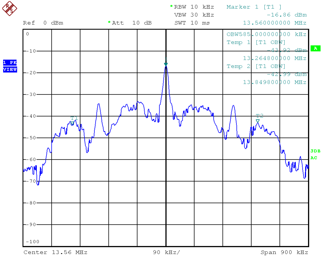
Figure 9: Chart of occupied bandwidth test
