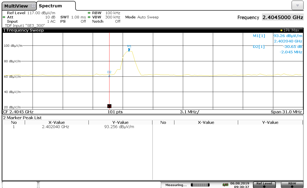
Figure 17: Chart of band-edge measurement on channel low
