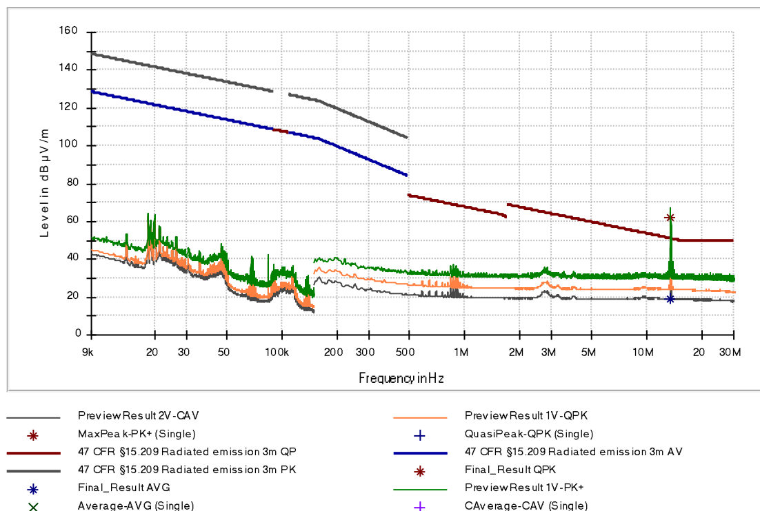
Figure 11: Chart of emissions test below 30 MHz without tag in position Z, antenna in line @ 3 m
