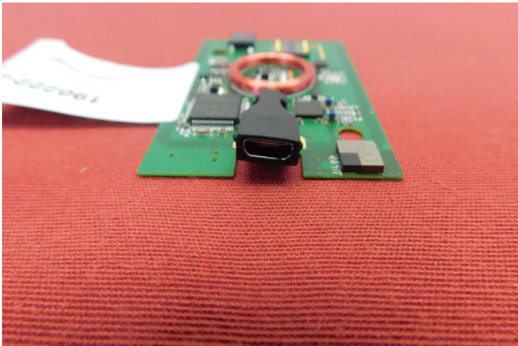
Picture 4: USB connector – front view
