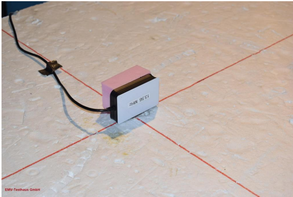
Picture 5: EUT-position 2
