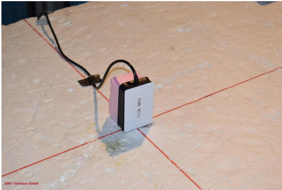
Picture 6: EUT-position 3
