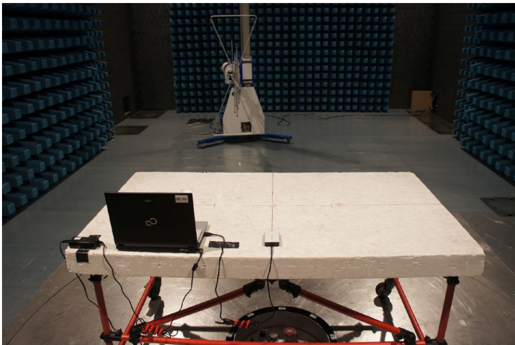
Picture 2: SAC, radiated emission test 30 MHz -1 GHz (front view)
