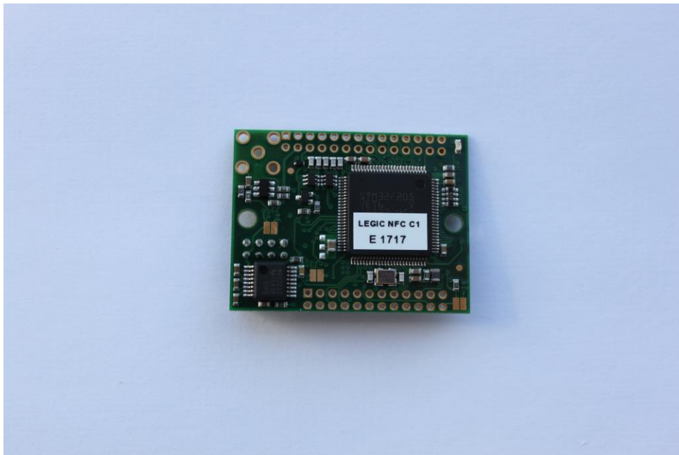
Picture 4: Top PCB – top side
