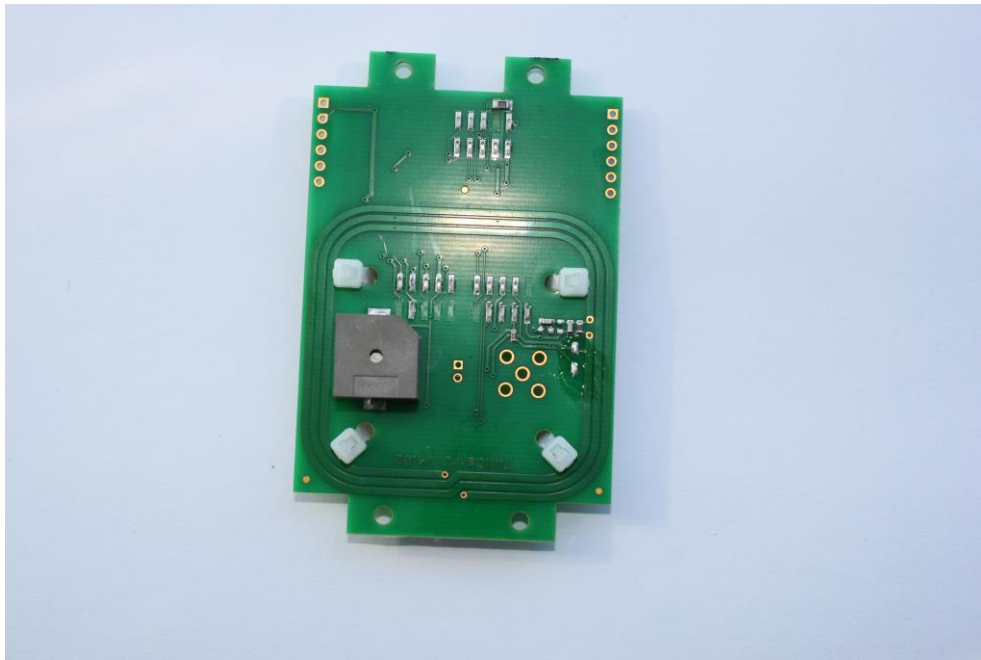
Picture 3: EUT – without top PCB
