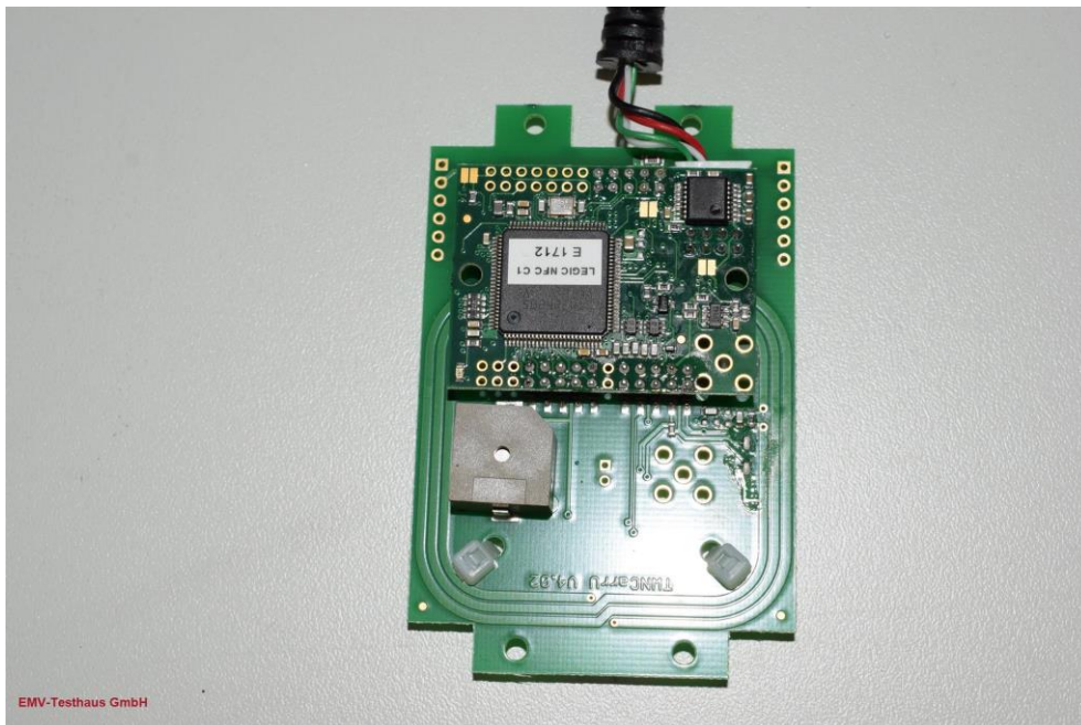
Picture 2: EUT – Open, bottom side
