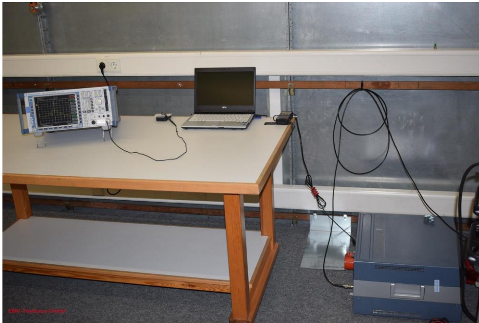
Picture 3: Test setup AC power line conducted emissions (front view)
