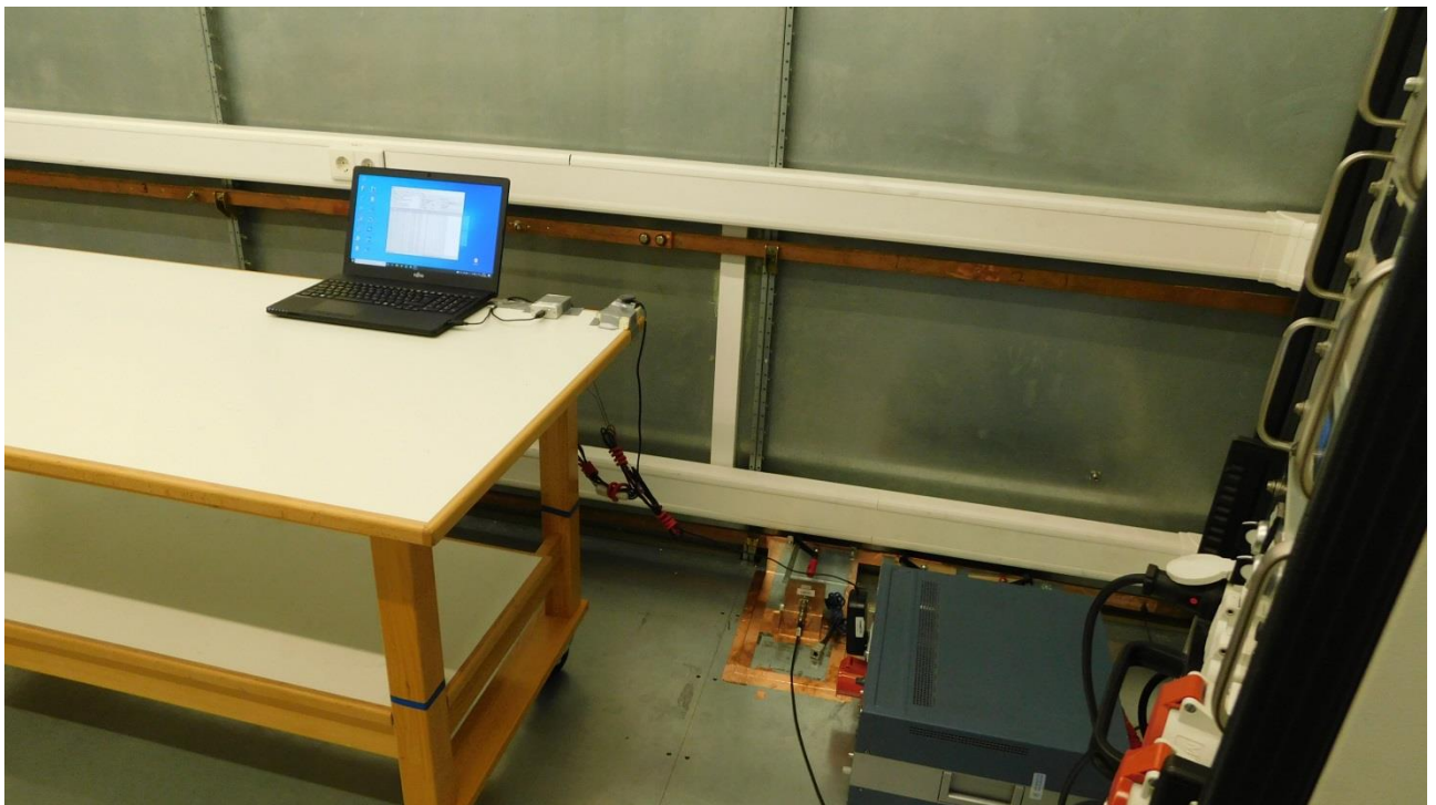
Picture 5: Test setup AC power line conducted emissions (front view)
