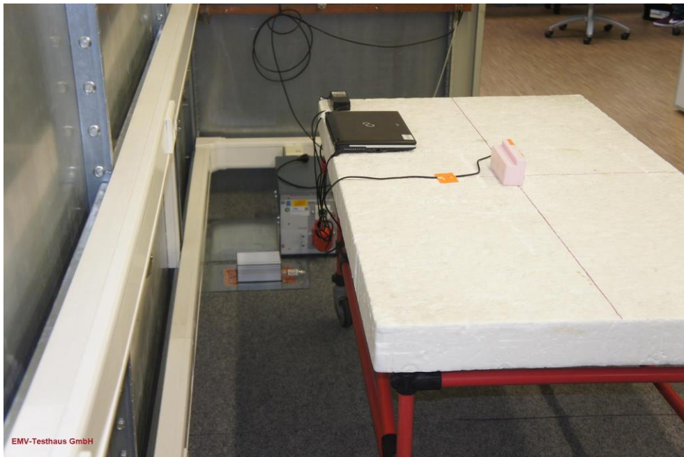
Picture 4: Test setup AC power line conducted emissions (rear view)
