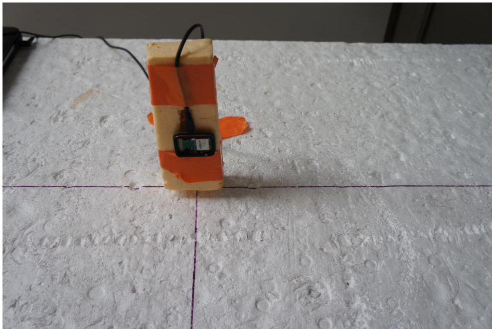
Picture 6: EUT-position 2
