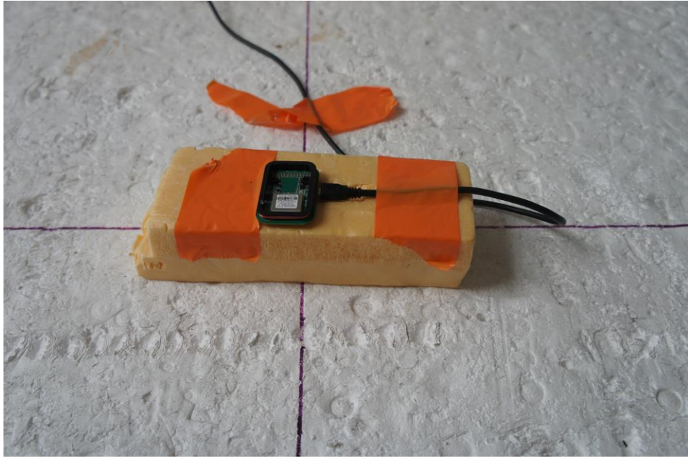
Picture 7: EUT-position 3
