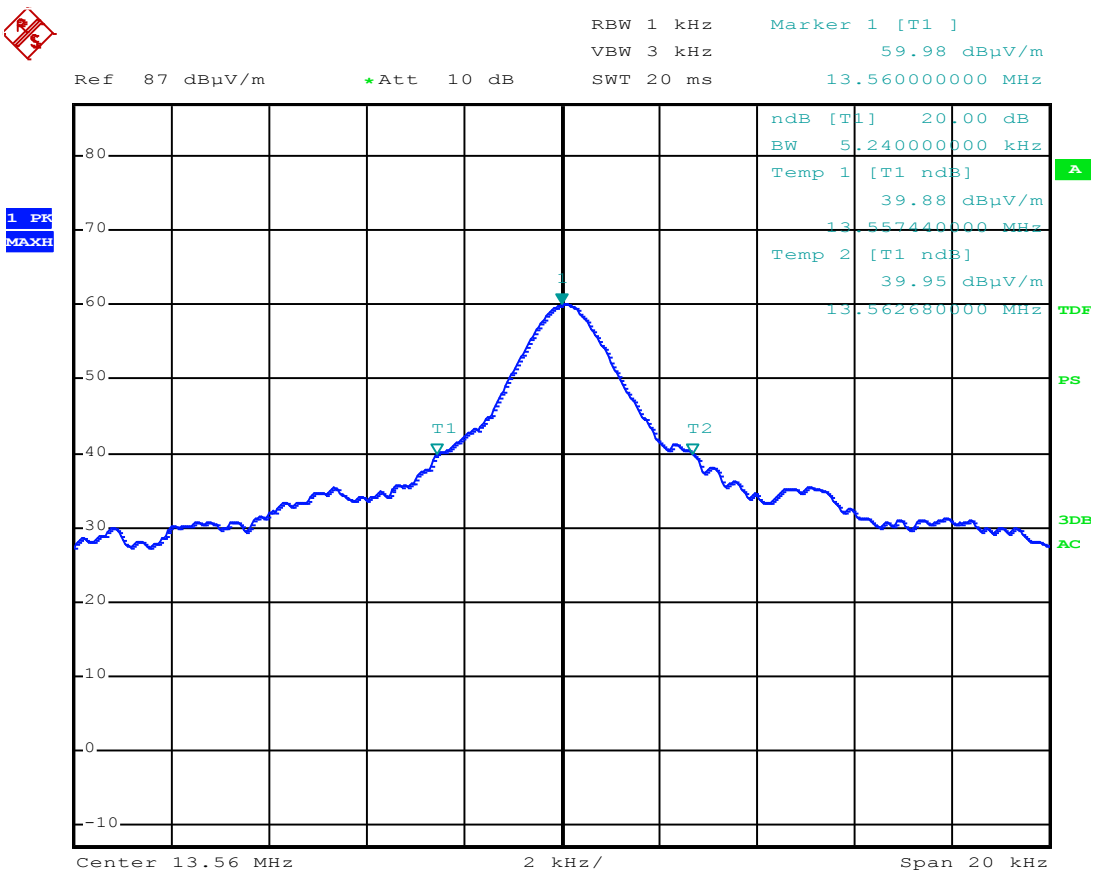
Picture 13: -20 dB emission bandwidth
