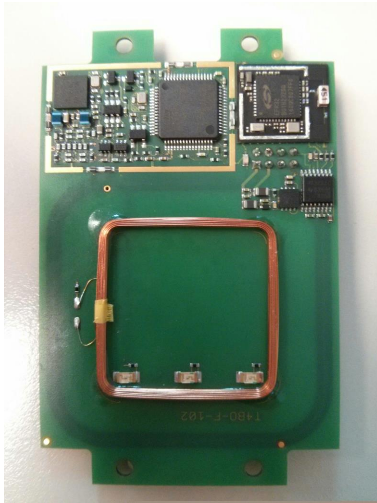
Picture 5: EUT - without RF shielding, with certified BLE module
