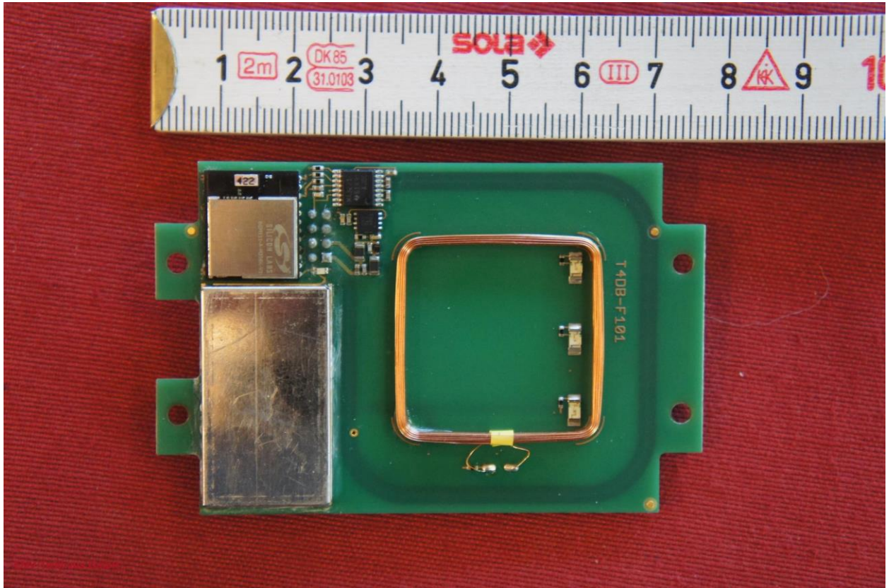
Picture 4: EUT - with RF shielding, with certified BLE module
