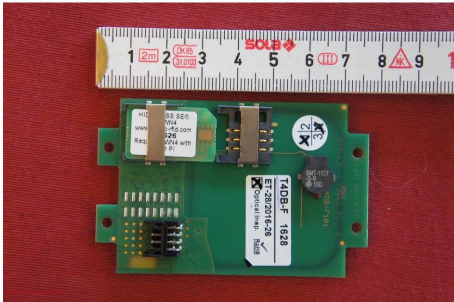
Picture 3: EUT - backside
