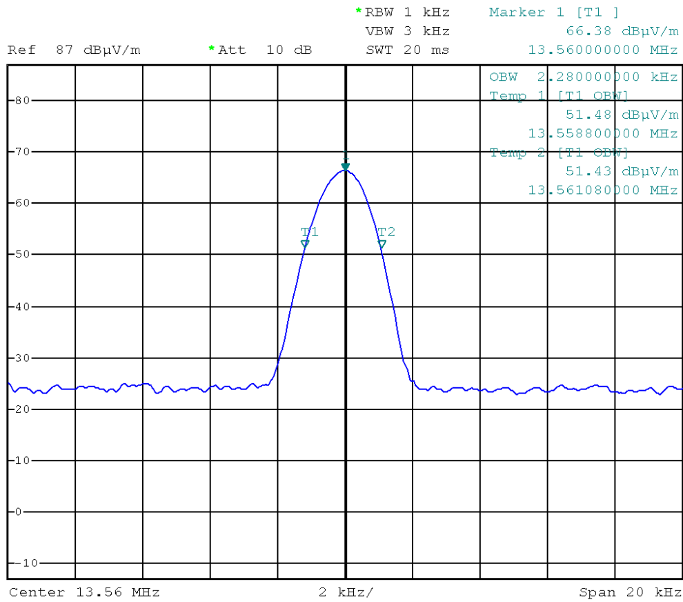
Picture 12: Occupied bandwidth (99 %)
