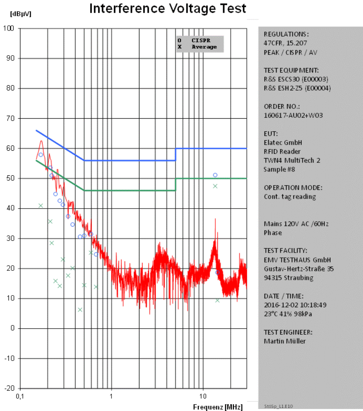
Picture 2: Graphic - Conducted emission on mains, phase 1 (without termination)
