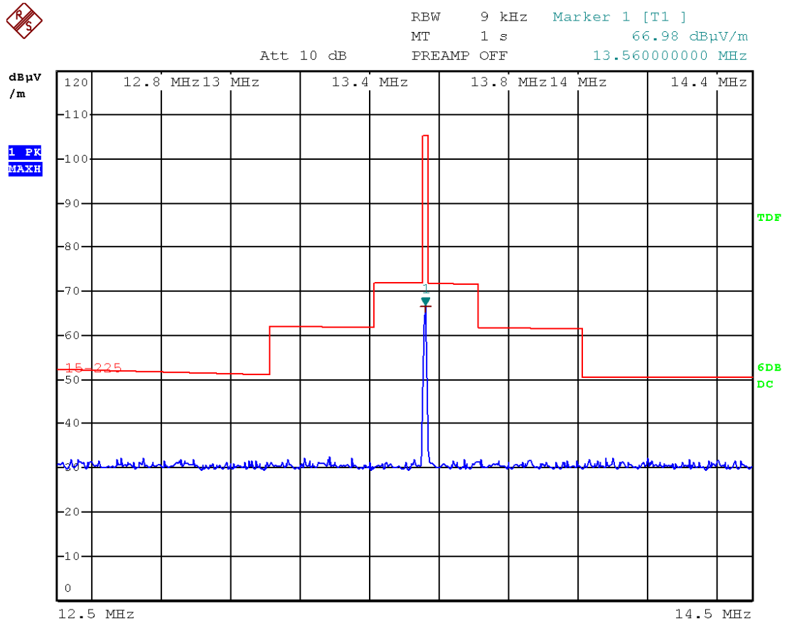
Picture 10: Spectrum mask for 13.56 MHz @ 3m distance
