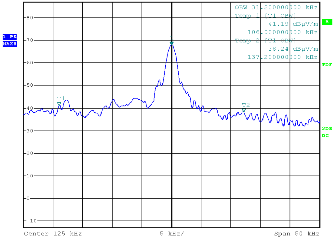
Picture 12: Occupied bandwidth (99 %)
