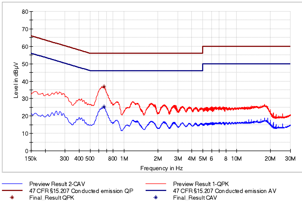
Figure 8: Chart of AC powerline conducted emissions on L1_sample with 50 Ω termination
