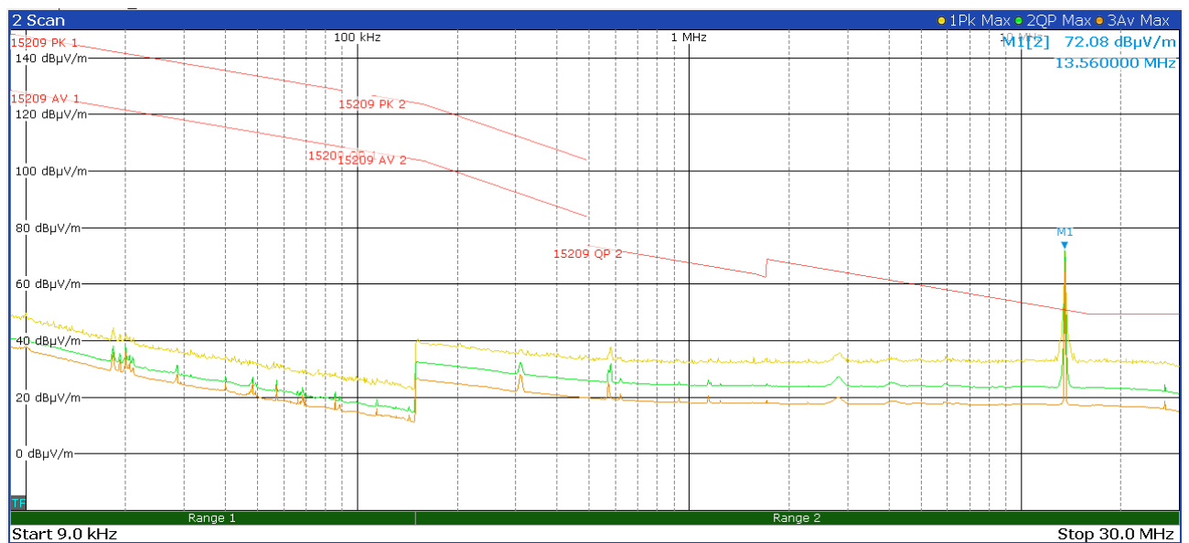
Figure 13: Chart of radiated emissions test below 30 MHz, EUT position Y, antenna polarization in line, without tag
