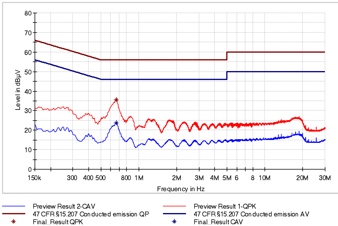
Figure 9: Chart of AC powerline conducted emissions on N_sample with 50 Ω termination
