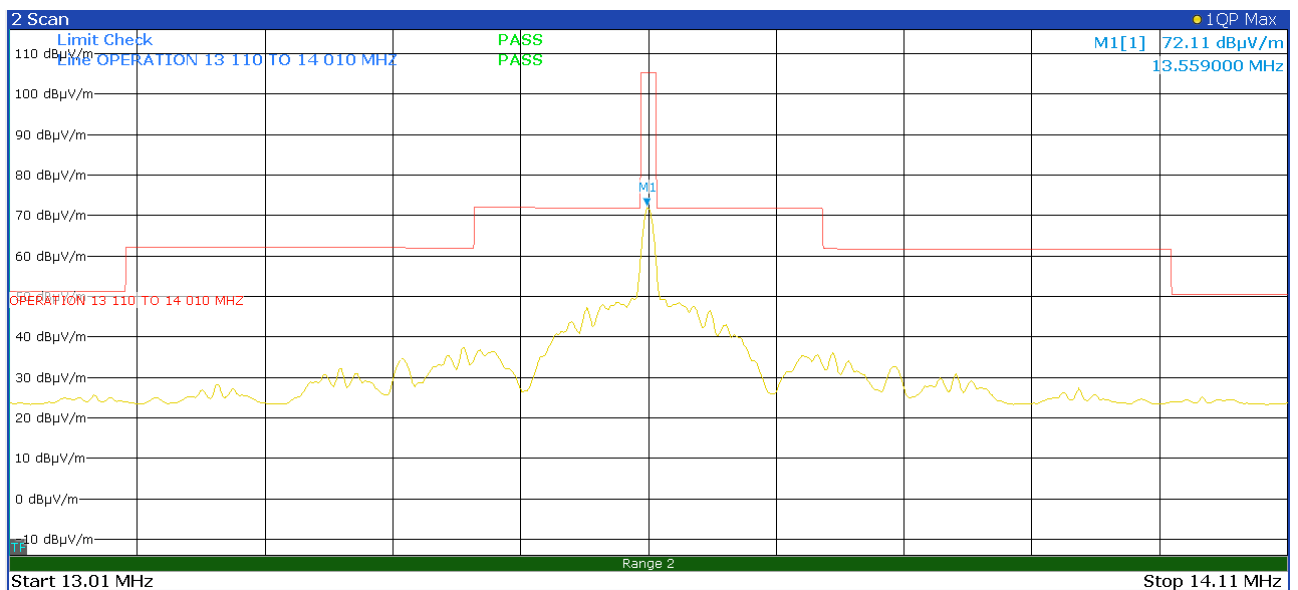
Figure 12: Chart of emission within the band 13.110 MHz to 14.010 MHz, EUT in position Y, without tag, antenna in line at 3 m distance
