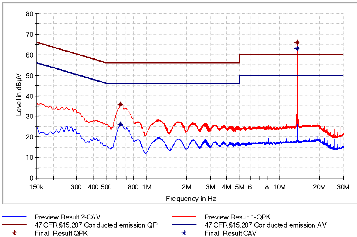
Figure 7: Chart of AC powerline conducted emissions on N_normal sample
