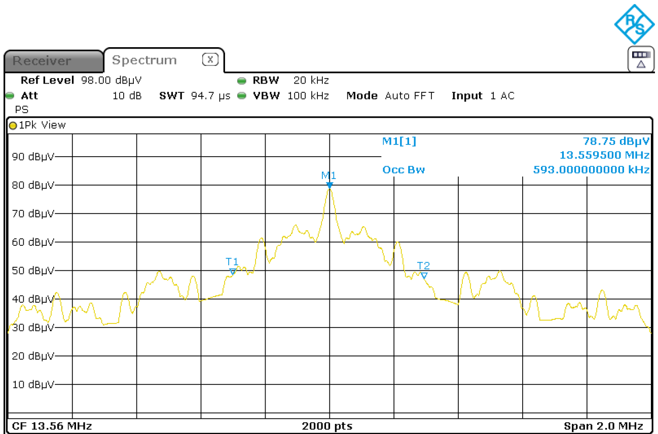
Figure 11: Chart of occupied bandwidth test, with tag
