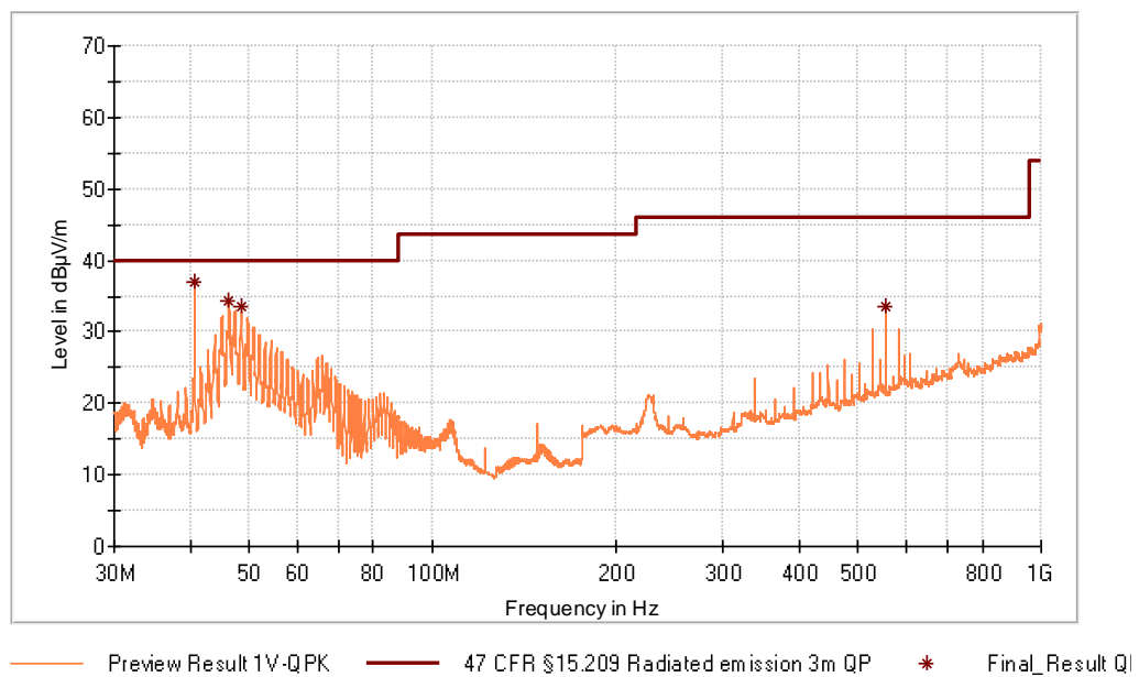
Figure 14: Chart of radiated emissions test from 30 MHz to 1 GHz, EUT position X, antenna polarization vertical, without tag
