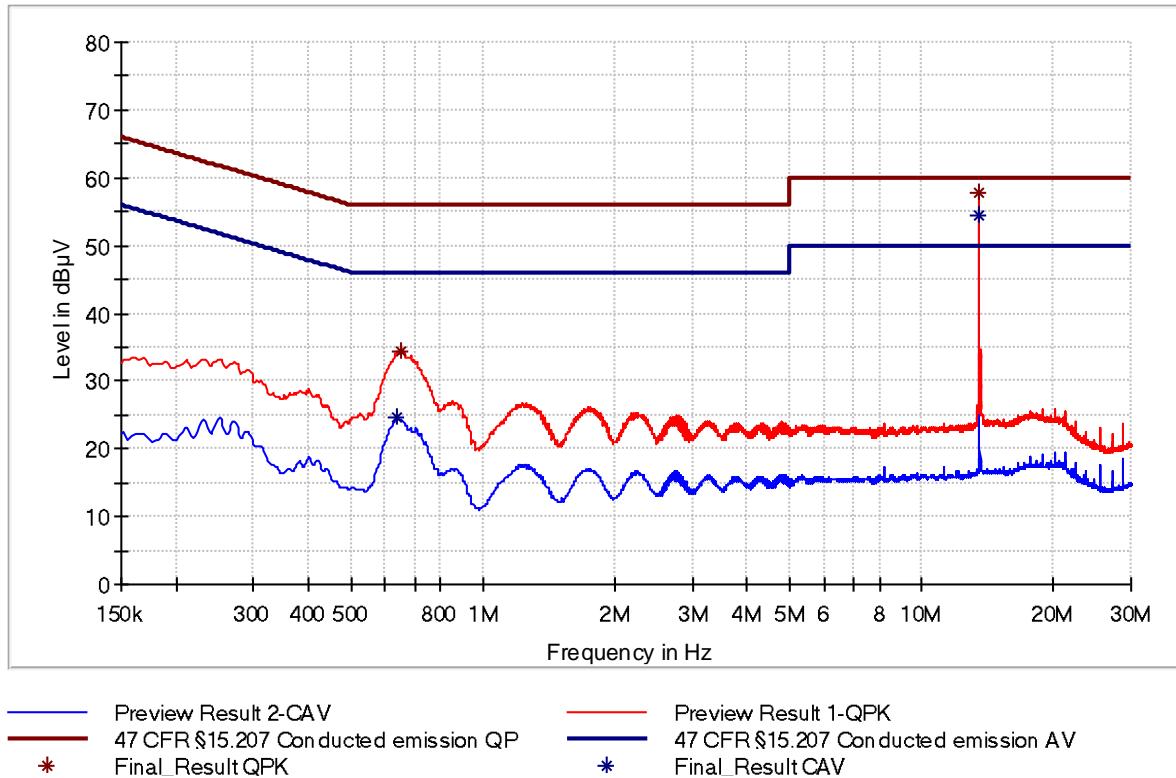
Figure 6: Chart of AC powerline conducted emissions on L1_normal sample
