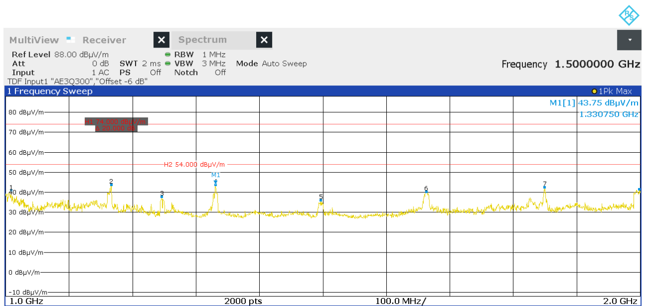
Figure 15: Chart of emissions test from 1 GHz to 2 GHz, EUT position Y, antenna polarization vertical, with tag
