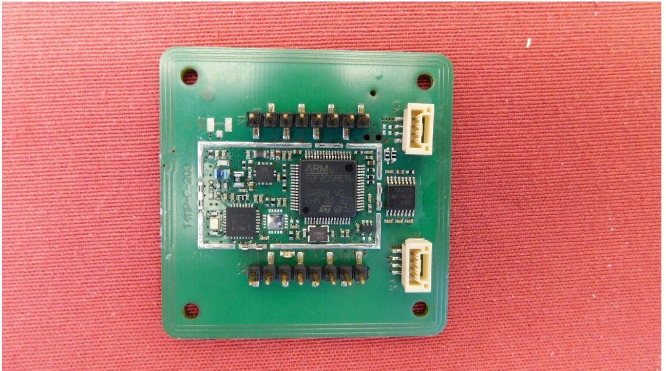
Picture 3: EUT – bottom side without shielding
