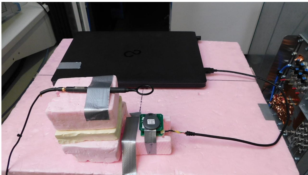
Picture 9: Bandwidth measurements
