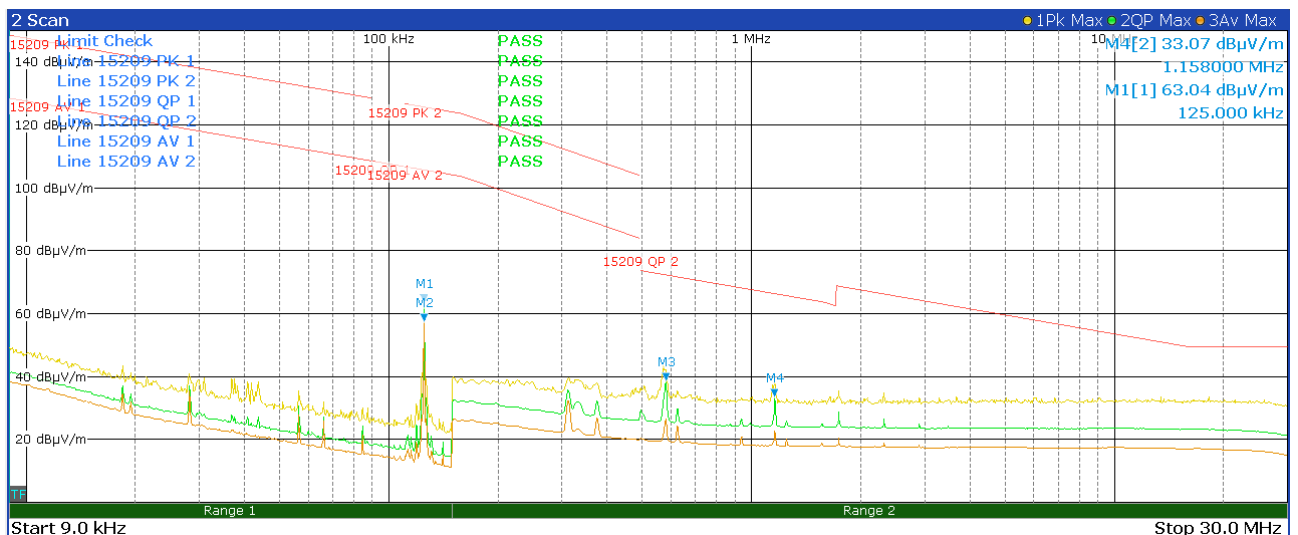
Figure 8: Chart of radiated emissions test below 30 MHz, EUT position Y, antenna polarization parallel, with tag
