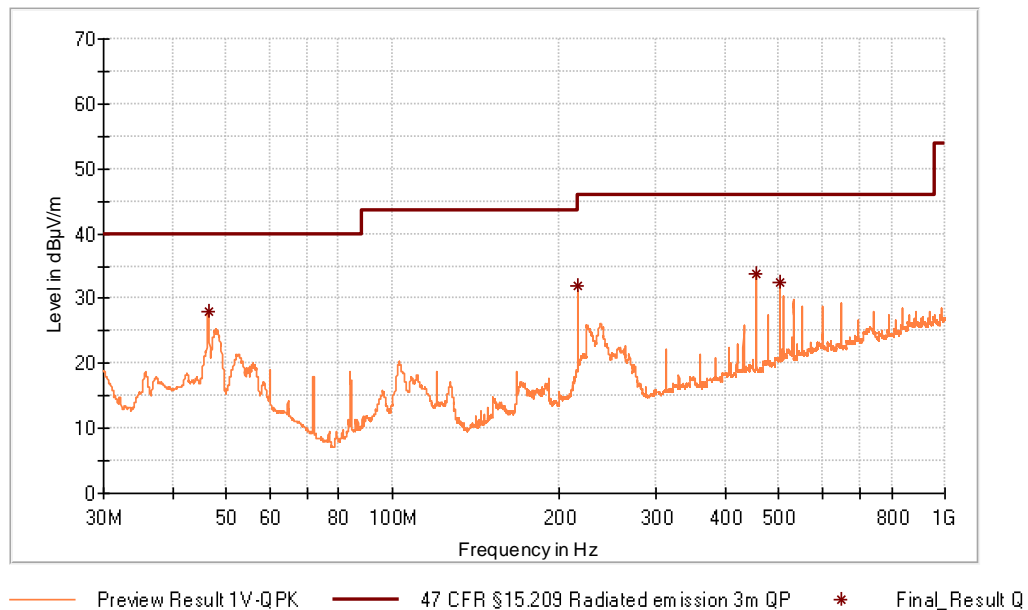
Figure 9: Chart of radiated emissions test from 30 MHz to 1 GHz, EUT position Z, without tag, antenna vertical
