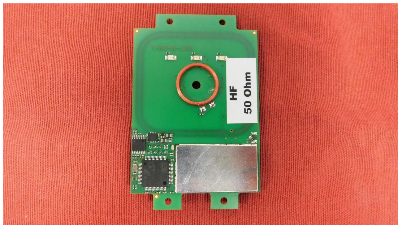
Picture 20: Top view of EUT with terminated antenna
