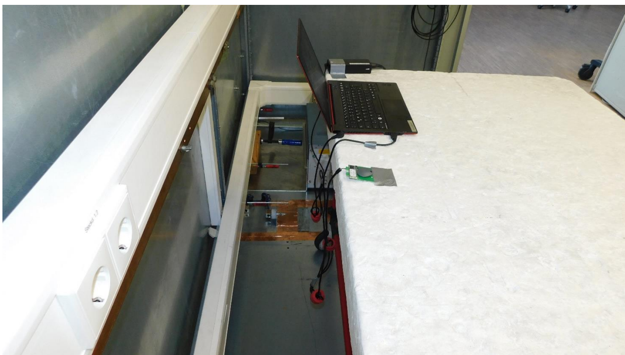
Picture 8: Test setup AC power line conducted emissions (rear view), USB
