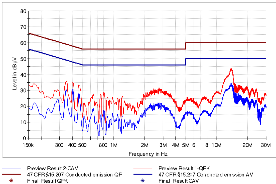
Figure 8: Chart of AC powerline conducted emissions on L1 – with termination, USB
