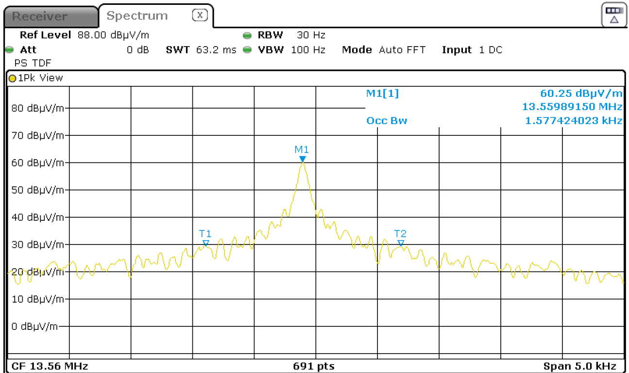
Figure 16: Chart of occupied bandwidth test, with tag, USB
