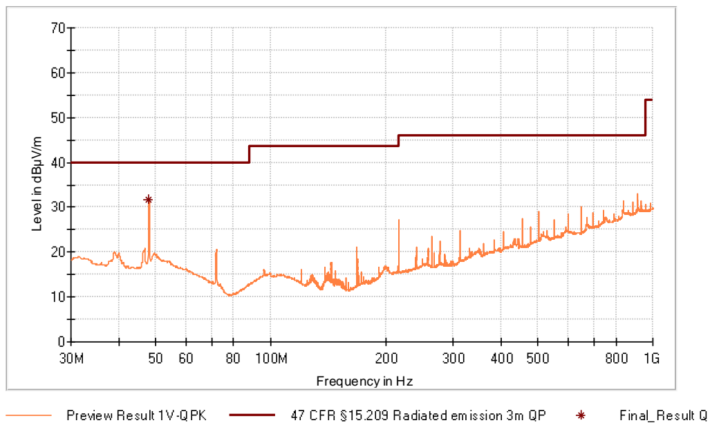
Figure 23: Chart of radiated emissions test from 30 MHz to 1 GHz, EUT position Y, antenna vertical, without tag, RS232
