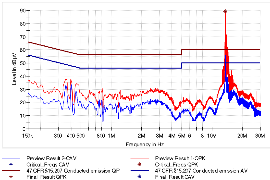
Figure 7: Chart of AC powerline conducted emissions on N – without termination, USB
