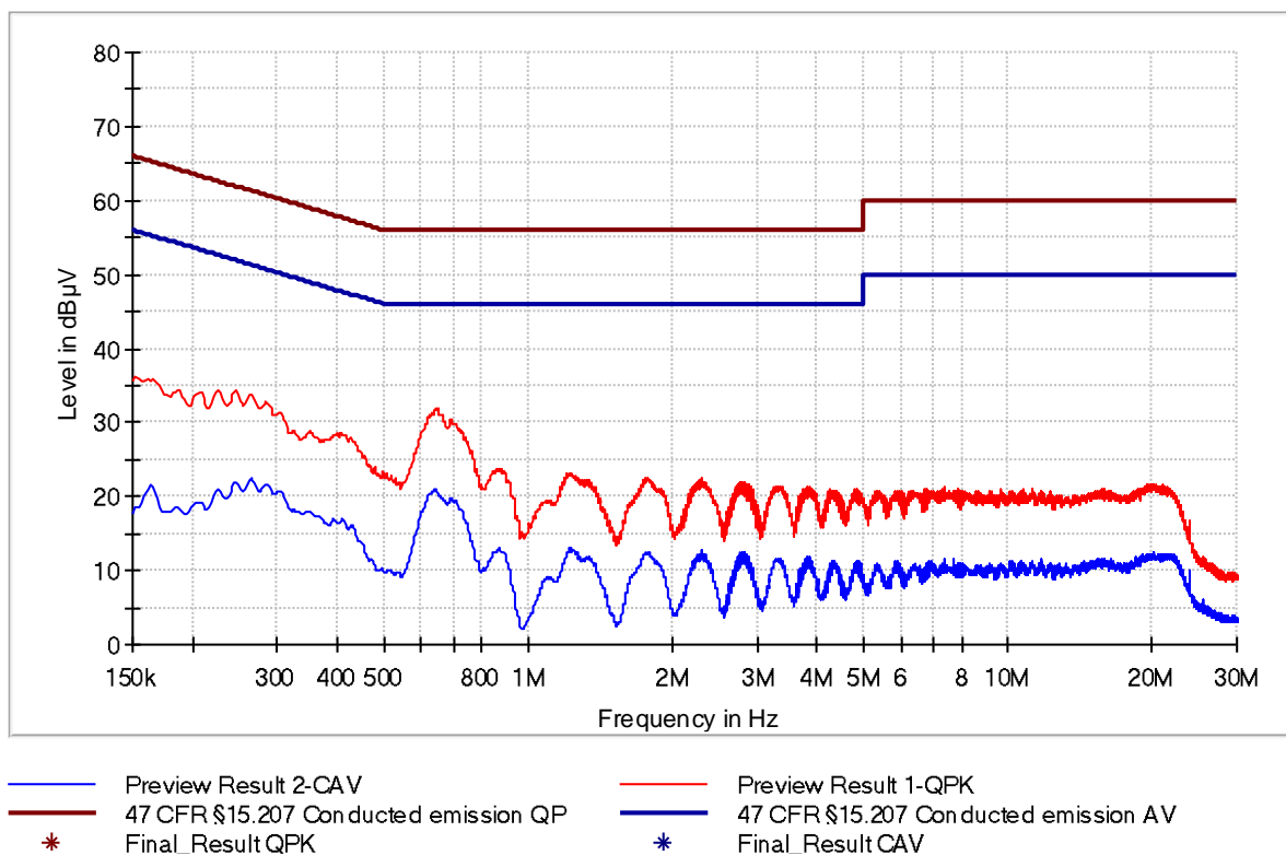
Figure 13: Chart of AC powerline conducted emissions on N – with termination, RS232
