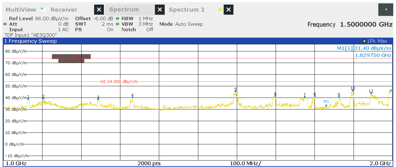
Figure 24: Chart of pre-measurement from 1 GHz to 2 GHz, EUT position X, with tag, antenna polarization vertical, USB
