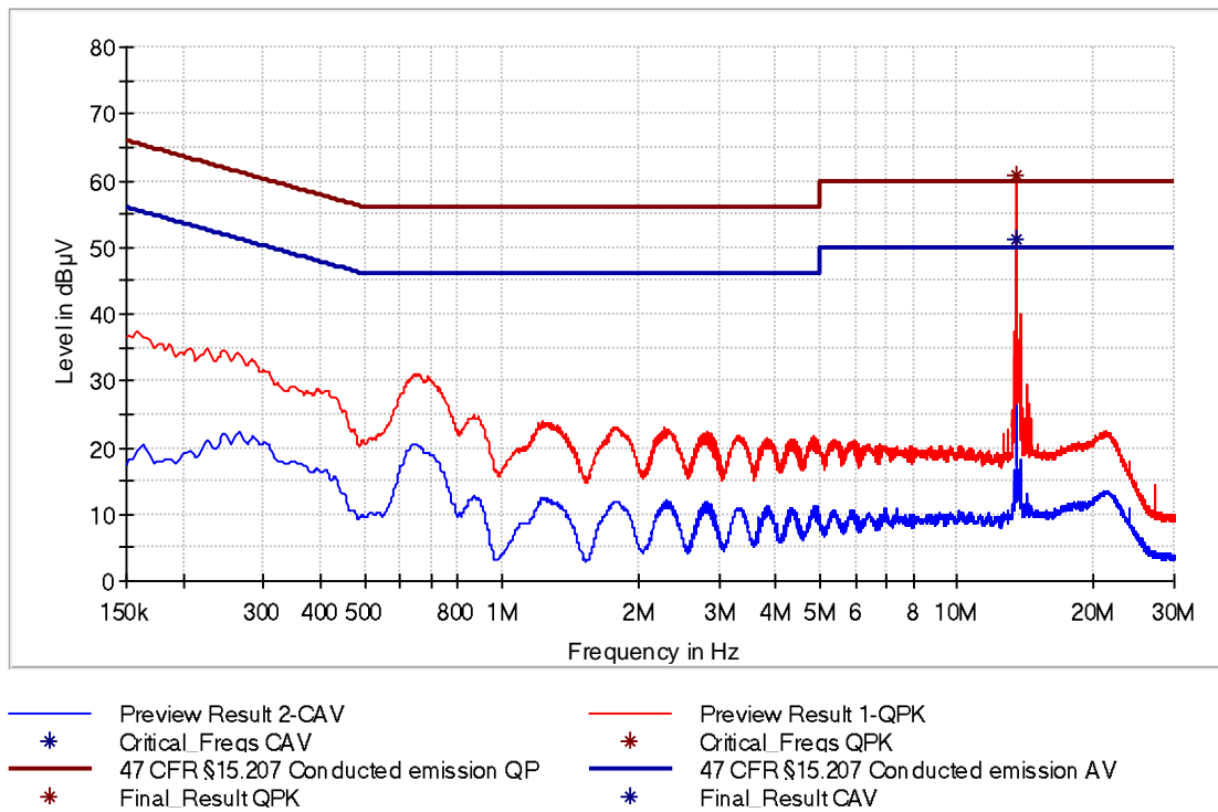
Figure 10: Chart of AC powerline conducted emissions on L1 – without termination, RS232
