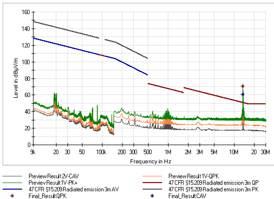
Figure 20: Chart of radiated emissions test below 30 MHz, EUT position X, antenna in line , without tag, USB
