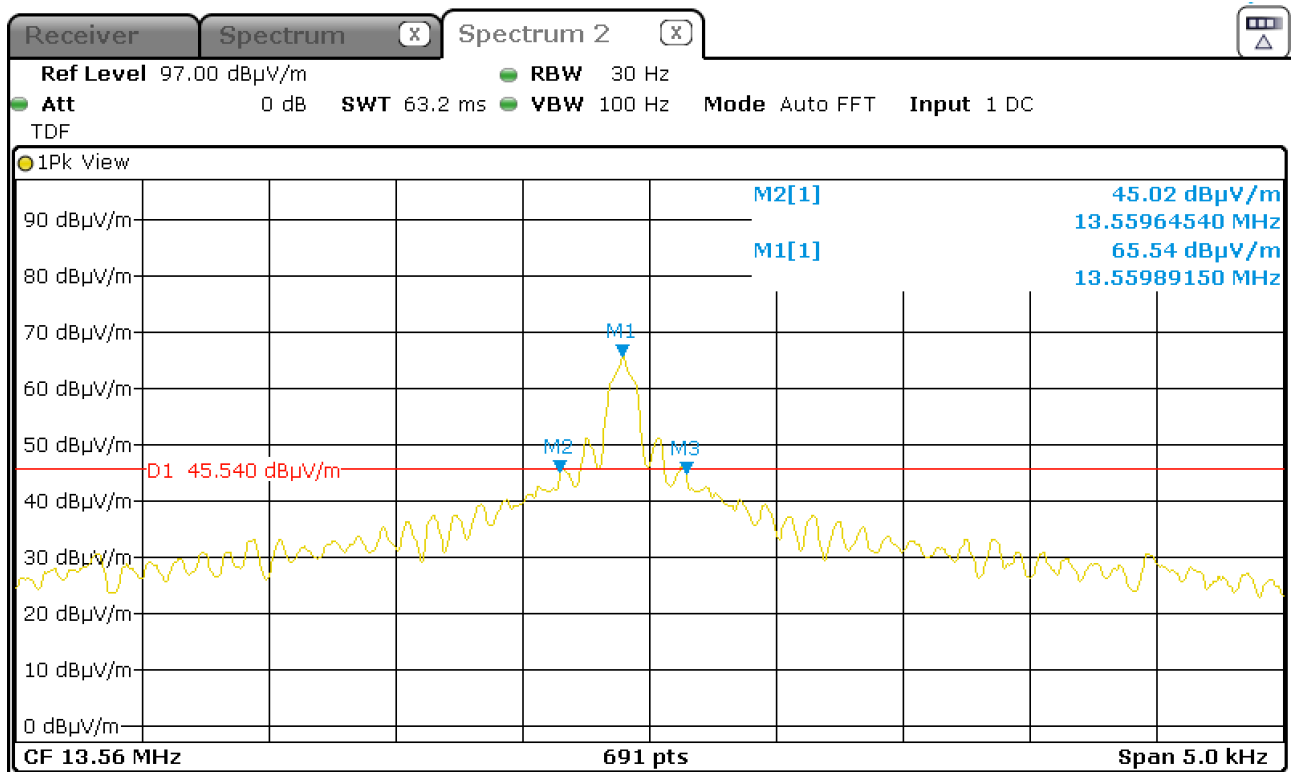
Figure 14: Chart of 20 dB bandwidth tests, without tag, USB
