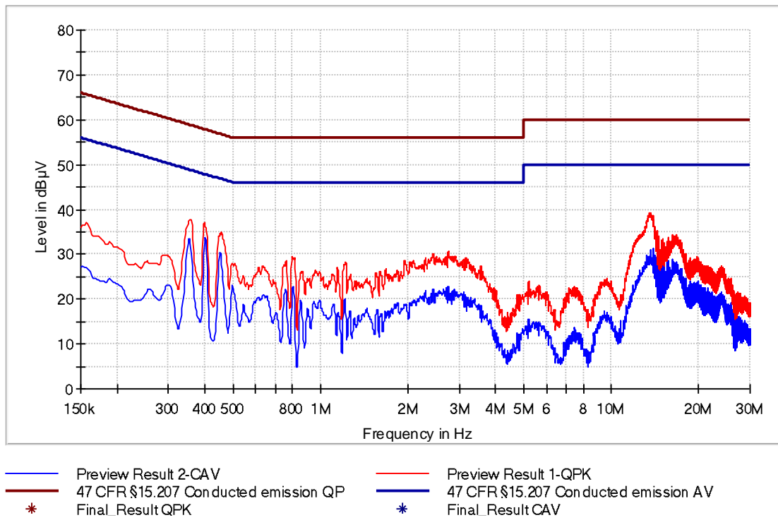
Figure 9: Chart of AC powerline conducted emissions on N – with termination, USB
