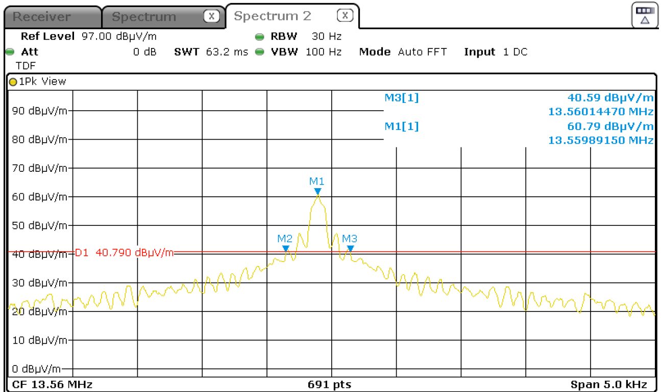
Figure 15: Chart of 20 dB bandwidth tests, without tag, RS232
