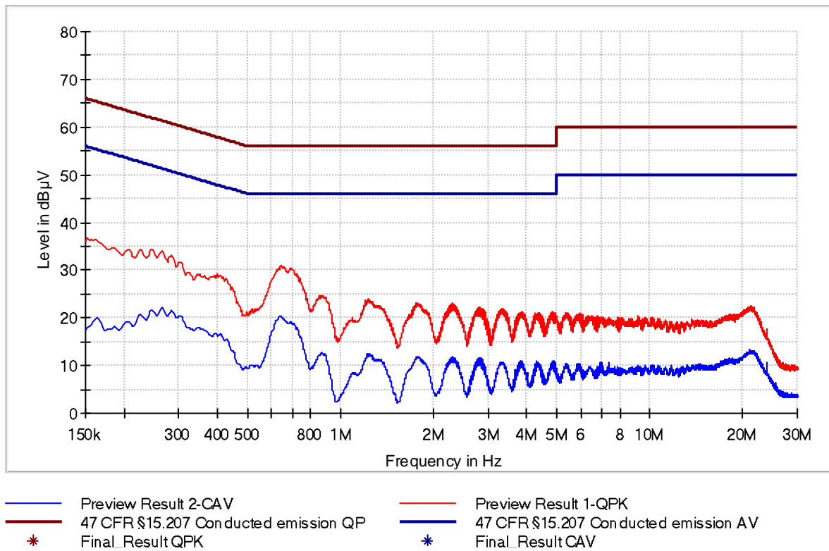
Figure 12: Chart of AC powerline conducted emissions on L1 – with termination, RS232
