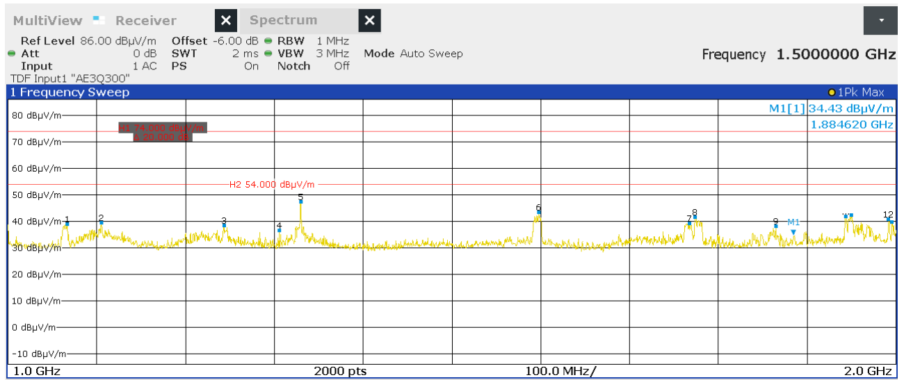
Figure 25: Chart of pre-measurement from 1 GHz to 2 GHz, EUT position Y, with tag, antenna polarization vertical, RS232
