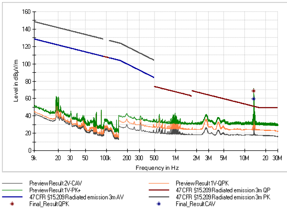
Figure 21: Chart of radiated emissions test below 30 MHz, EUT position Z, antenna in line , without tag, RS232
