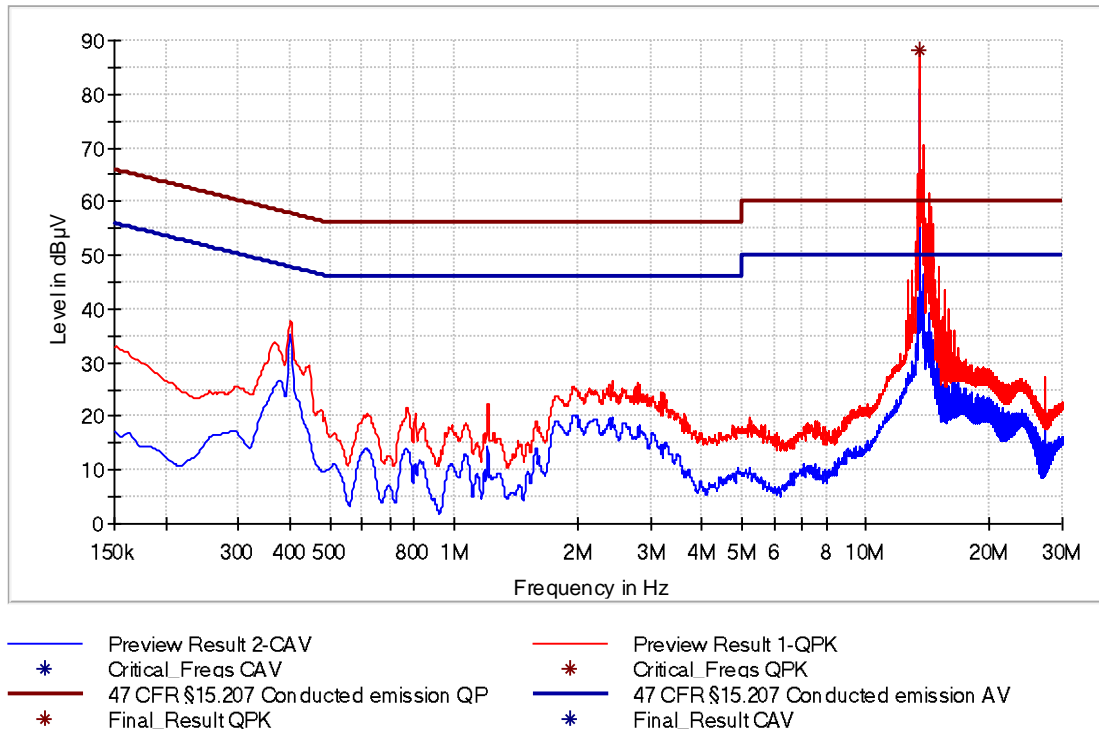
Figure 6: Chart of AC powerline conducted emissions on L1 – without termination, USB
