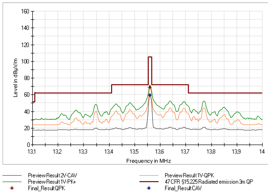
Figure 19: Chart of emission within the band 13.110 MHz to 14.010 MHz, EUT in position Z, without tag, antenna in line, RS232 at 3 m distance
