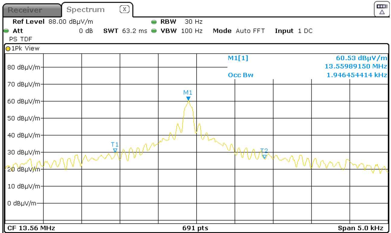
Figure 17: Chart of occupied bandwidth test, without tag, RS232
