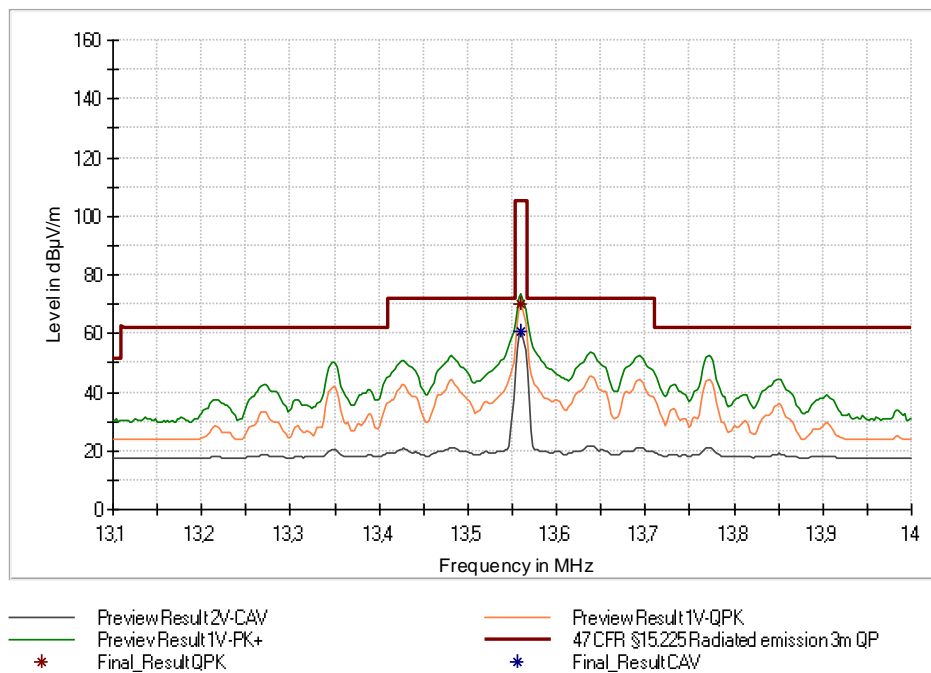
Figure 18: Chart of emission within the band 13.110 MHz to 14.010 MHz, EUT in position X, without tag, antenna in line, USB at 3 m distance
