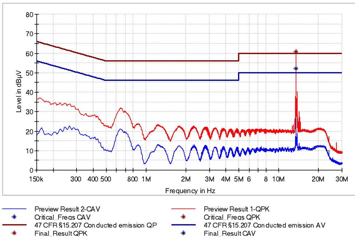
Figure 11: Chart of AC powerline conducted emissions on N – without termination, RS232
