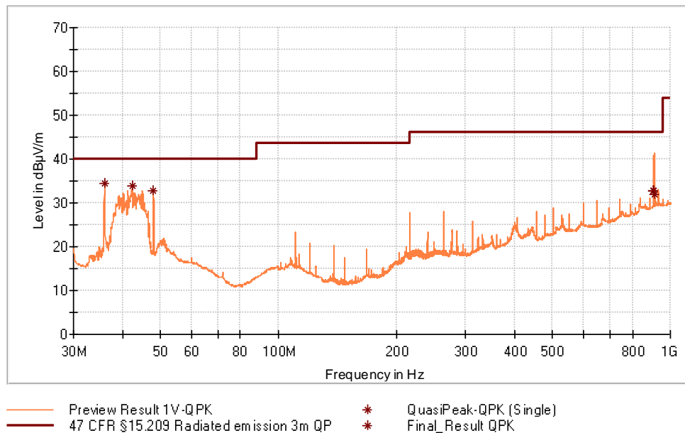
Figure 22: Chart of radiated emissions test from 30 MHz to 1 GHz, EUT position X, antenna vertical, with tag, USB
