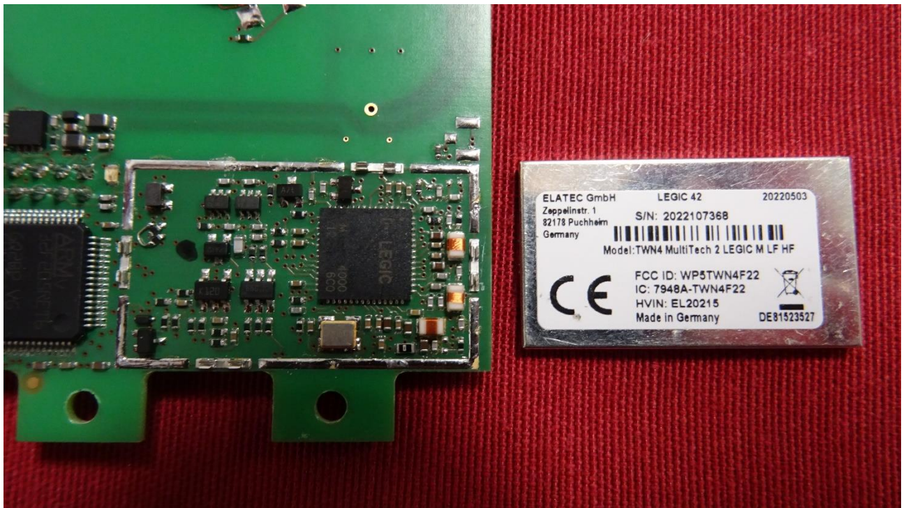
Picture 5: EUT without shielding – detailed view
