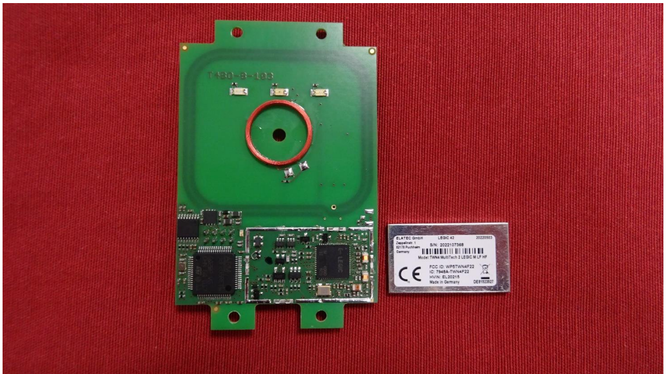
Picture 4: EUT without shielding – front view
