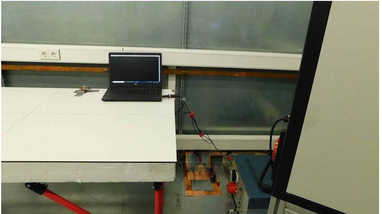
Picture 9: Test setup AC power line conducted emissions (front view), RS232
