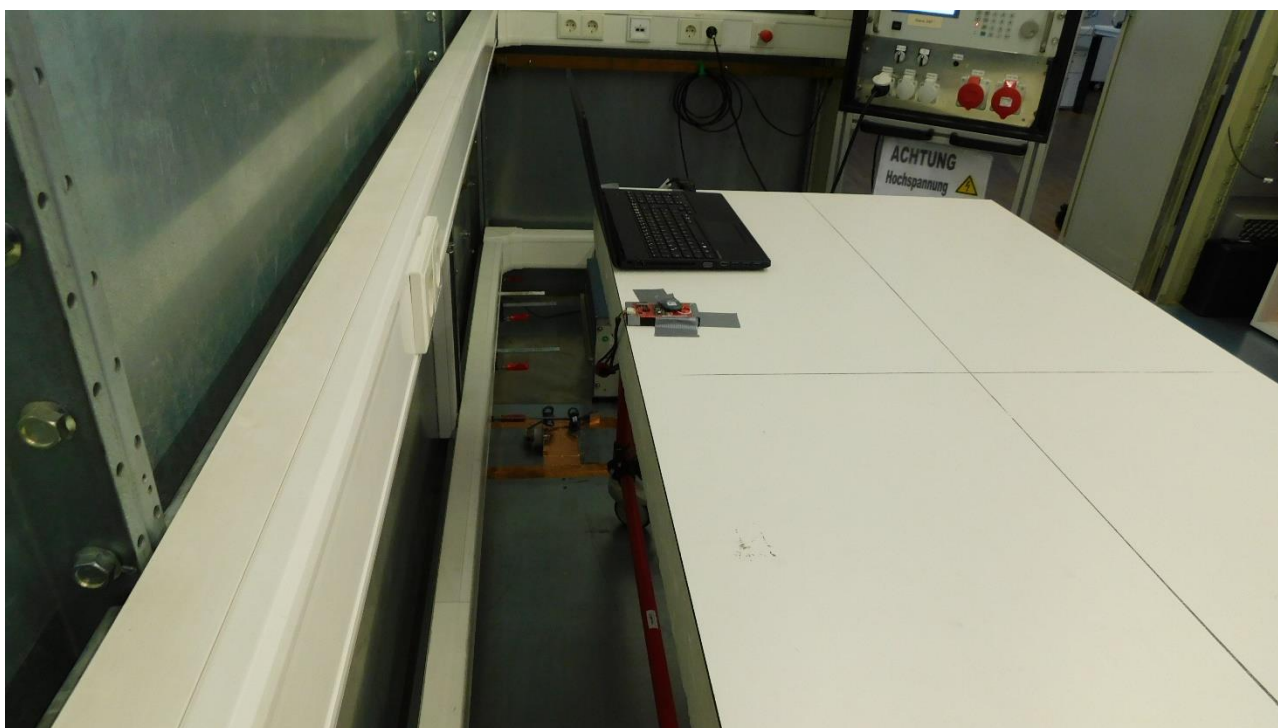
Picture 10: Test setup AC power line conducted emissions (rear view), RS232
