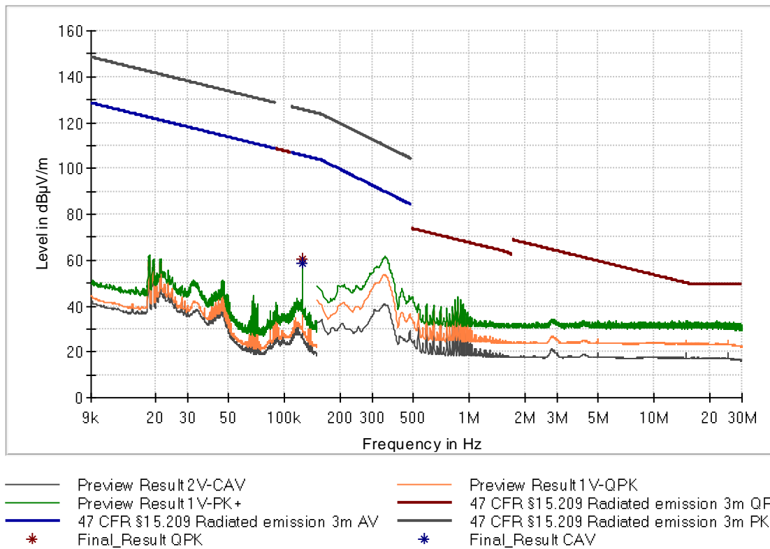
Figure 13: Chart of emissions test below 30 MHz, EUT position Z, without tag, antenna in line at 3 m, USB
