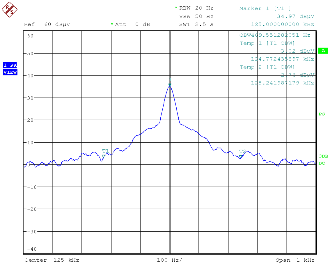
Figure 12: Chart of occupied bandwidth test, without tag, RS232
