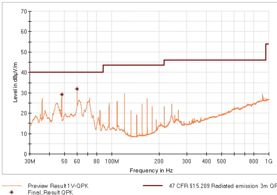
Figure 15: Chart of emissions test from 30 MHz to 1 GHz, EUT position Z, with tag, antenna vertical, at 3 m, USB
