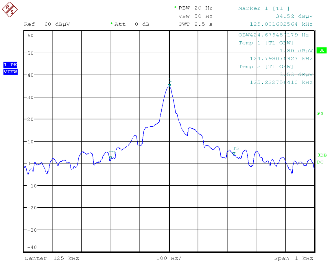
Figure 11: Chart of occupied bandwidth test, without tag, USB
