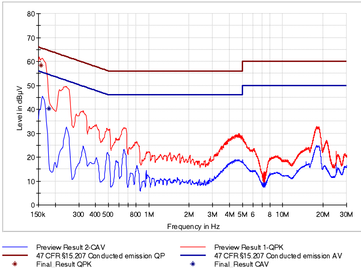
Figure 5: Chart of AC power-line conducted emissions test – phase L1, USB
