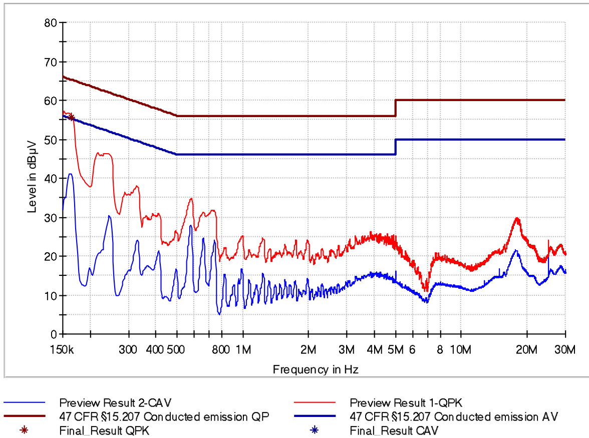
Figure 7: Chart of AC power-line conducted emissions test – phase N, USB
