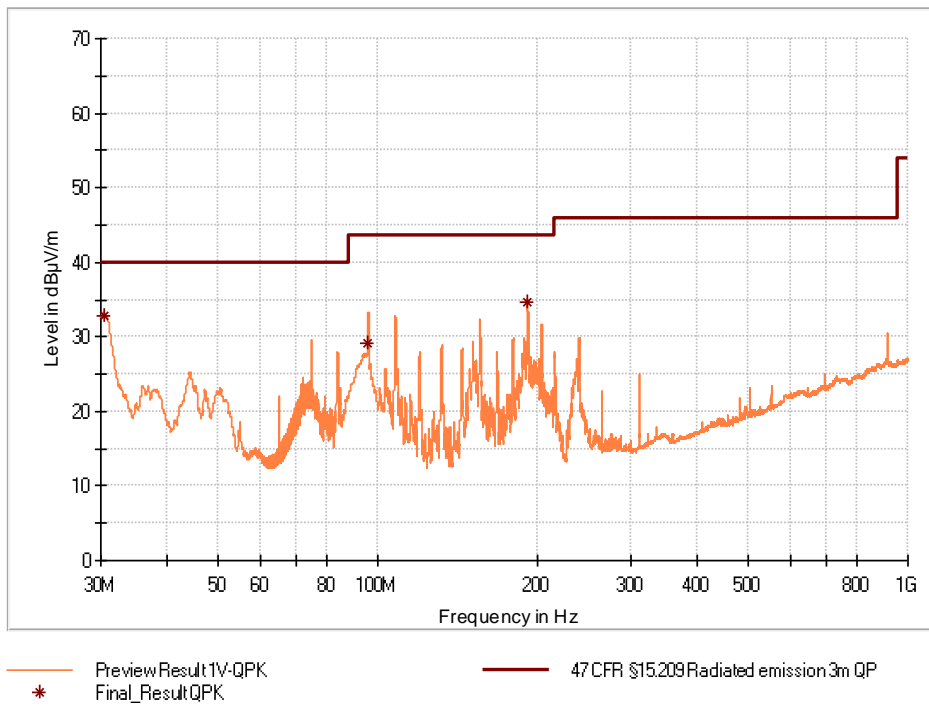
Figure 16: Chart of emissions test from 30 MHz to 1 GHz, EUT position Z, with tag, antenna vertical, at 3 m, RS232
