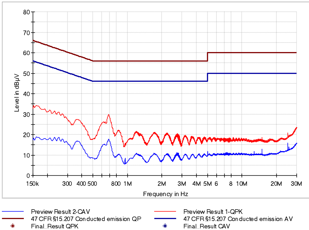
Figure 9: Chart of AC power-line conducted emissions test – phase L1, RS232
