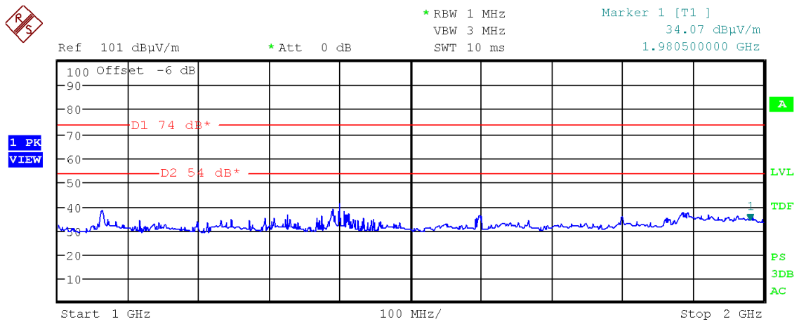
Figure 17: Chart of emissions test from 1 GHz to 2 GHz, EUT position X, without tag, antenna horizontal, at 3 m, USB
