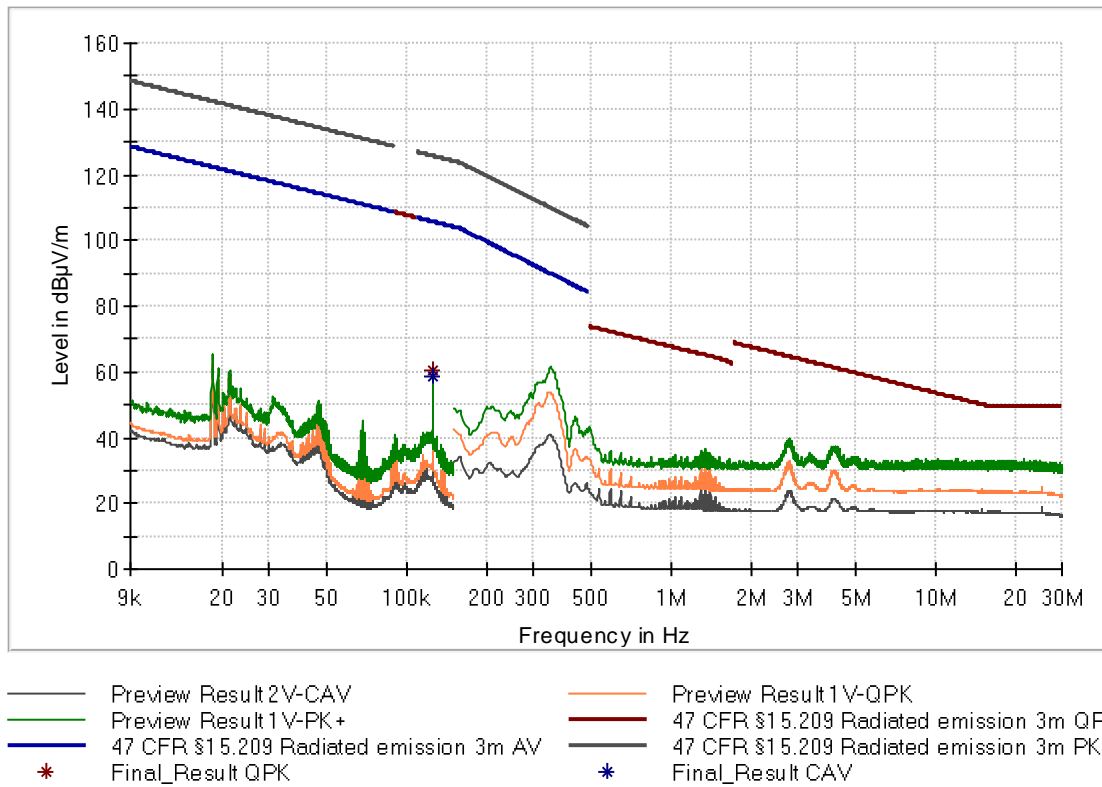
Figure 14: Chart of emissions test below 30 MHz, EUT position Z, without tag, antenna in line at 3 m, RS232
