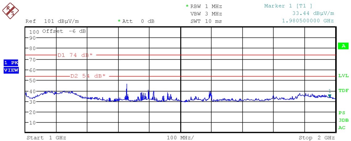
Figure 18: Chart of emissions test from 1 GHz to 2 GHz, EUT position X, without tag, antenna horizontal, at 3 m, RS232
