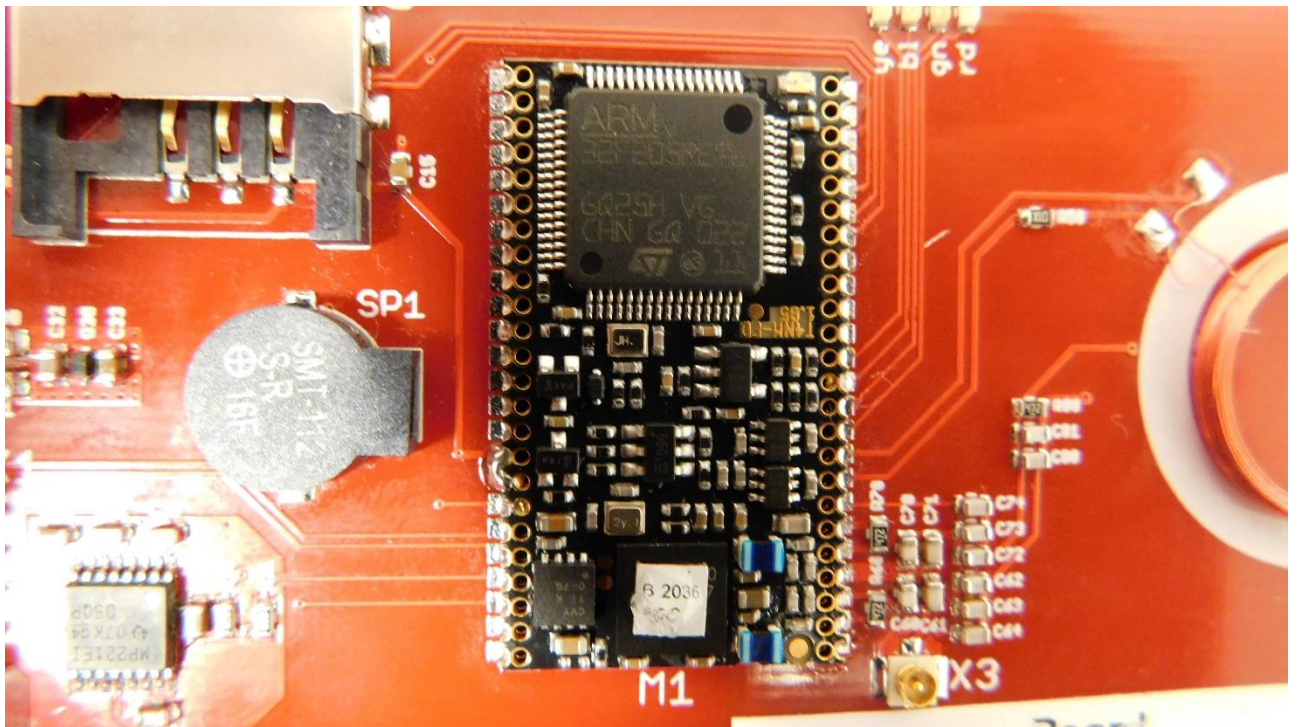
Picture 3: EUT - top view
