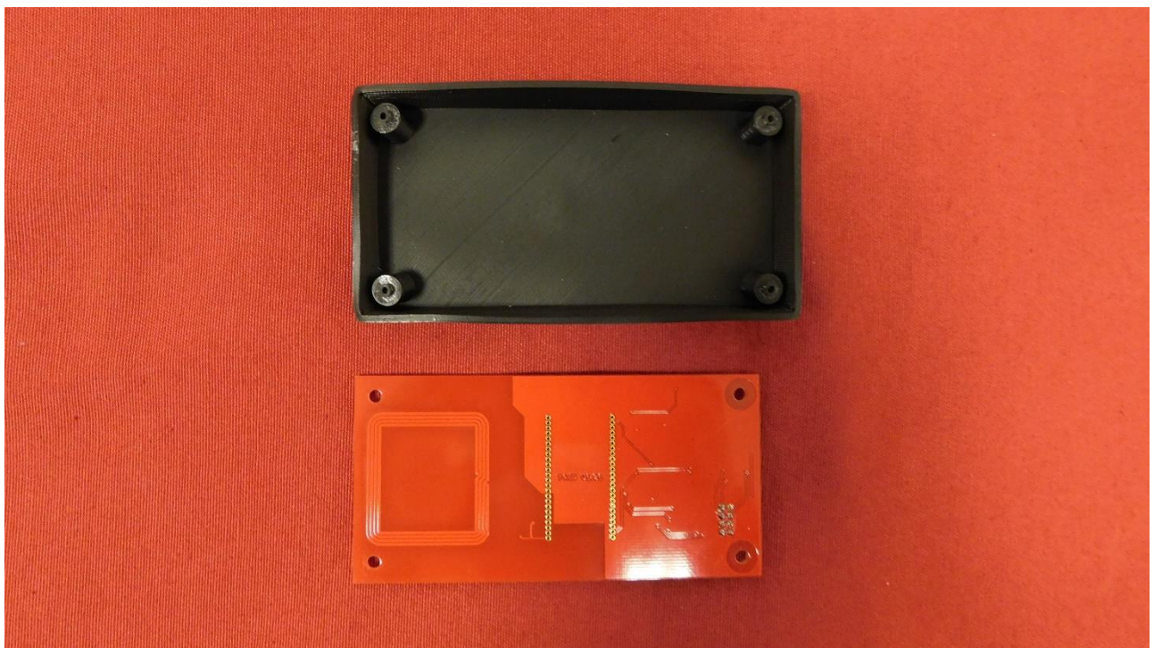
Picture 2: EUT on reference board – rear view
