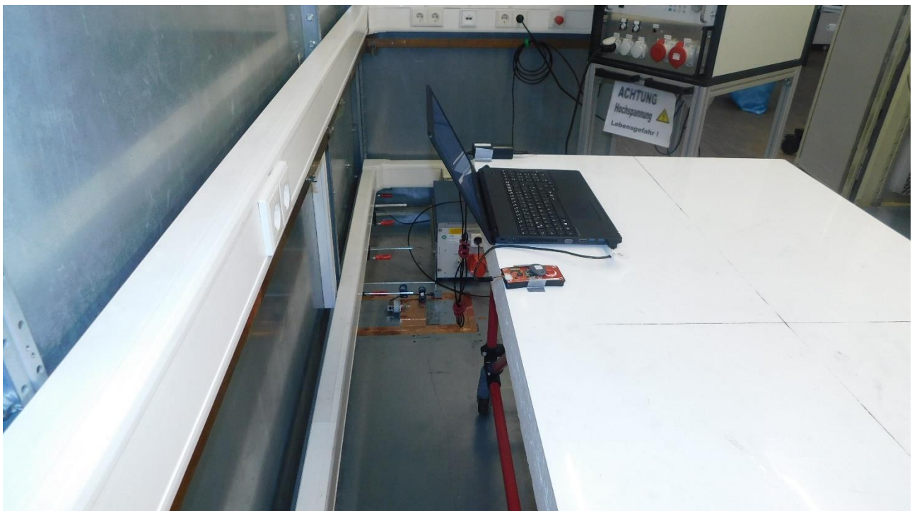
Picture 8: Test setup AC power line conducted emissions (rear view), USB
