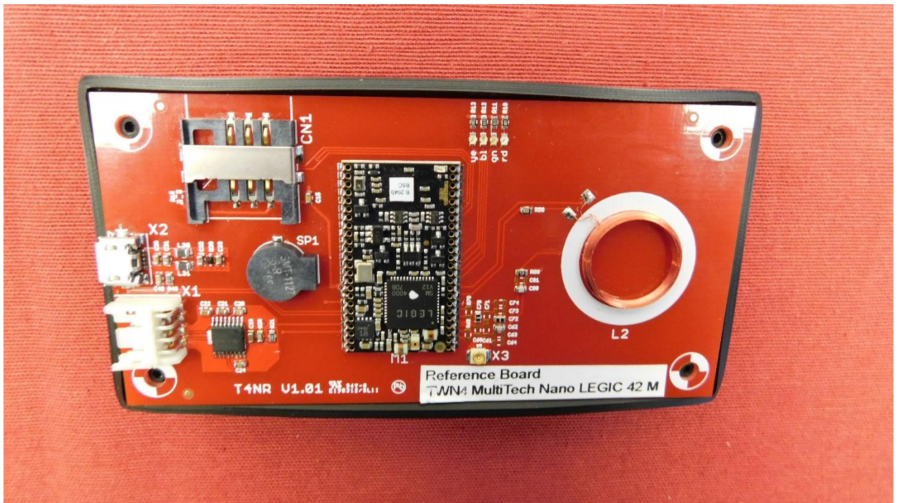
Picture 1: EUT on evaluation board – front view
