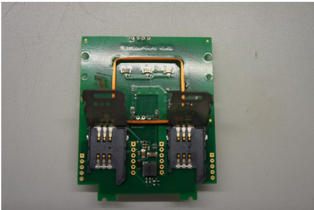
Picture 6: PCB top side (card slots open)
