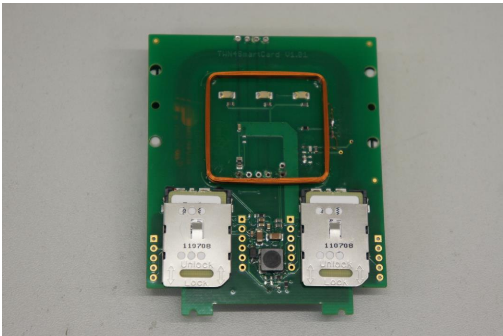
Picture 2: PCB top side
