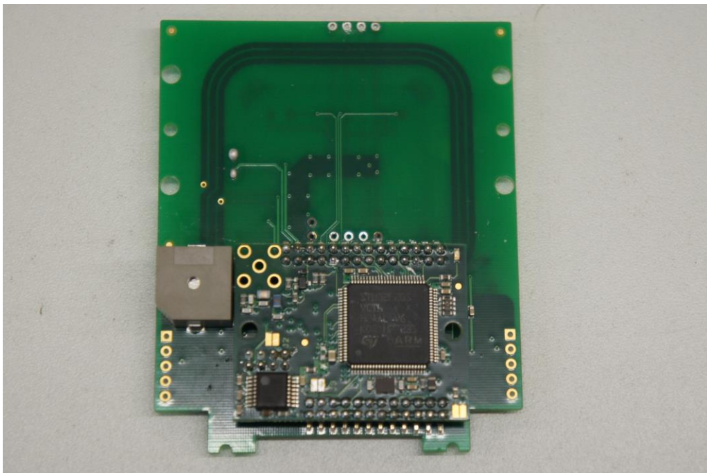
Picture 4: PCB bottom side (without card reader)
