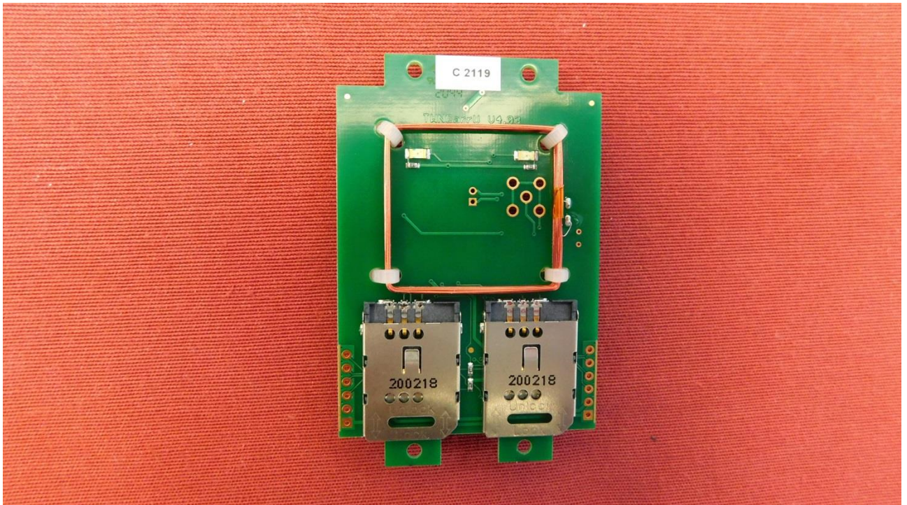
Picture 2: EUT – back side, without shielding
