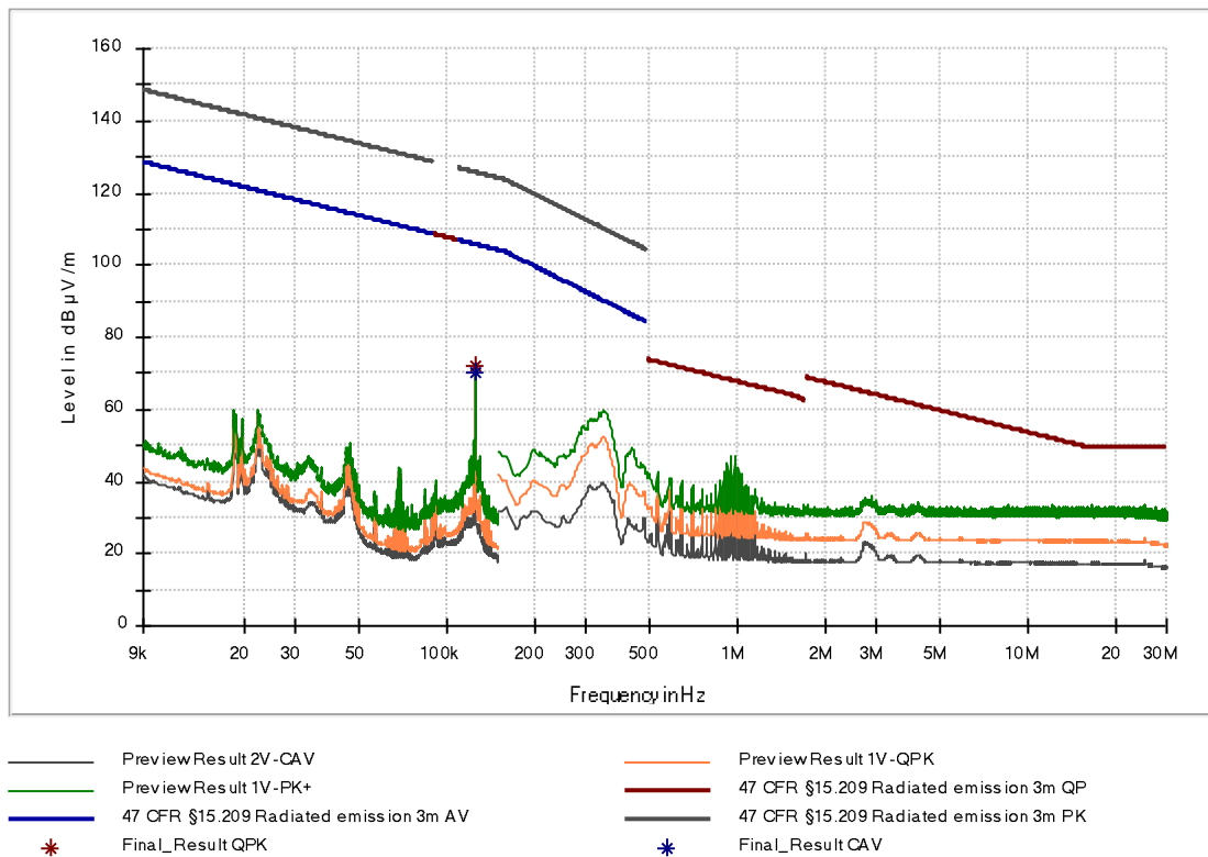
Figure 10: Chart of emissions test below 30 MHz, EUT position Z, without tag, antenna in line at 3 m
