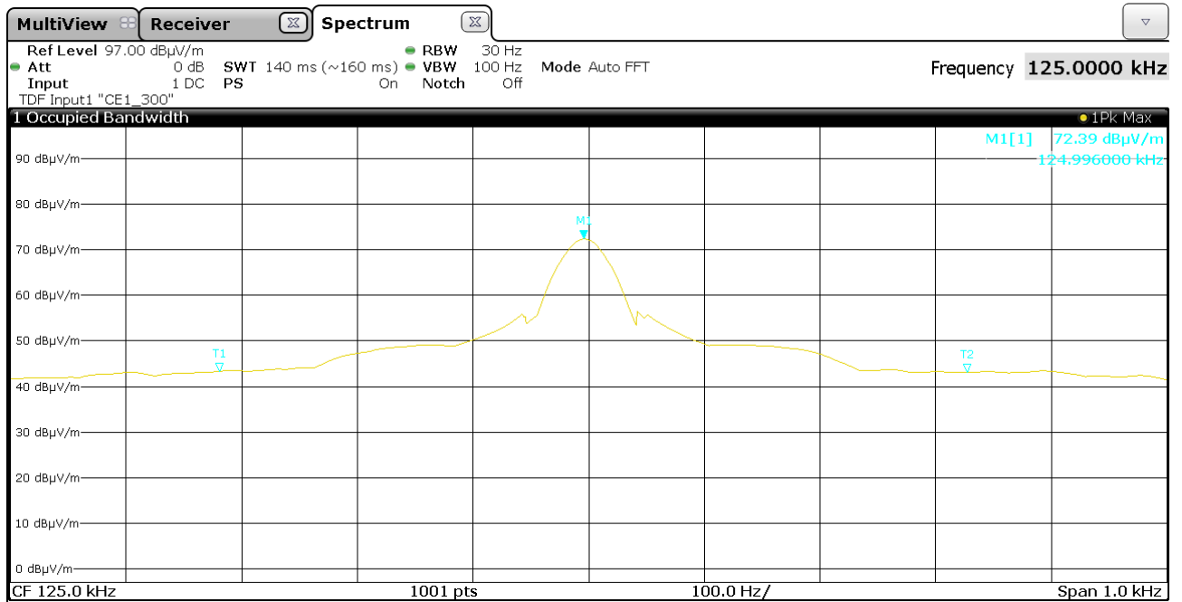
Figure 9: Chart of occupied bandwidth test, without tag
