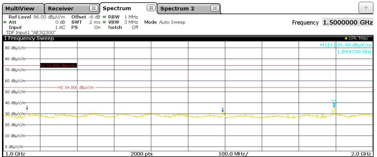
Figure 12: Chart of emissions test from 1 GHz to 2 GHz, EUT position X, with tag, antenna horizontal, at 3 m
