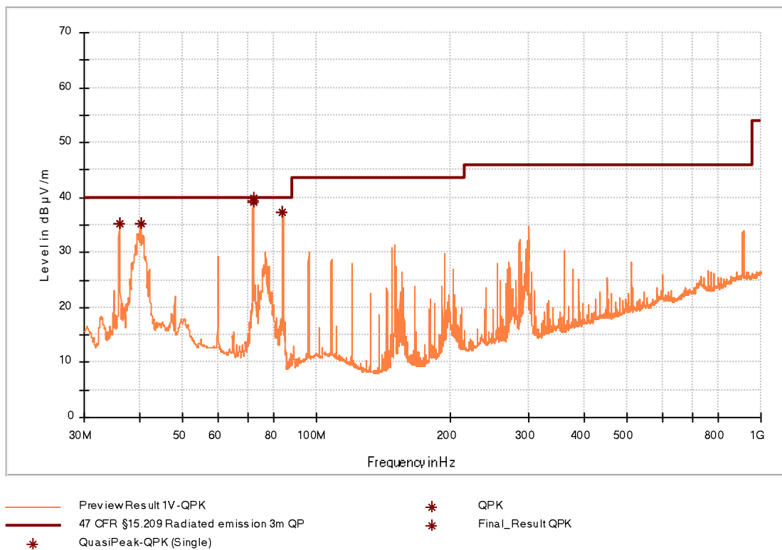
Figure 11: Chart of emissions test from 30 MHz to 1 GHz, EUT position Y, with tag, antenna vertical, at 3 m
