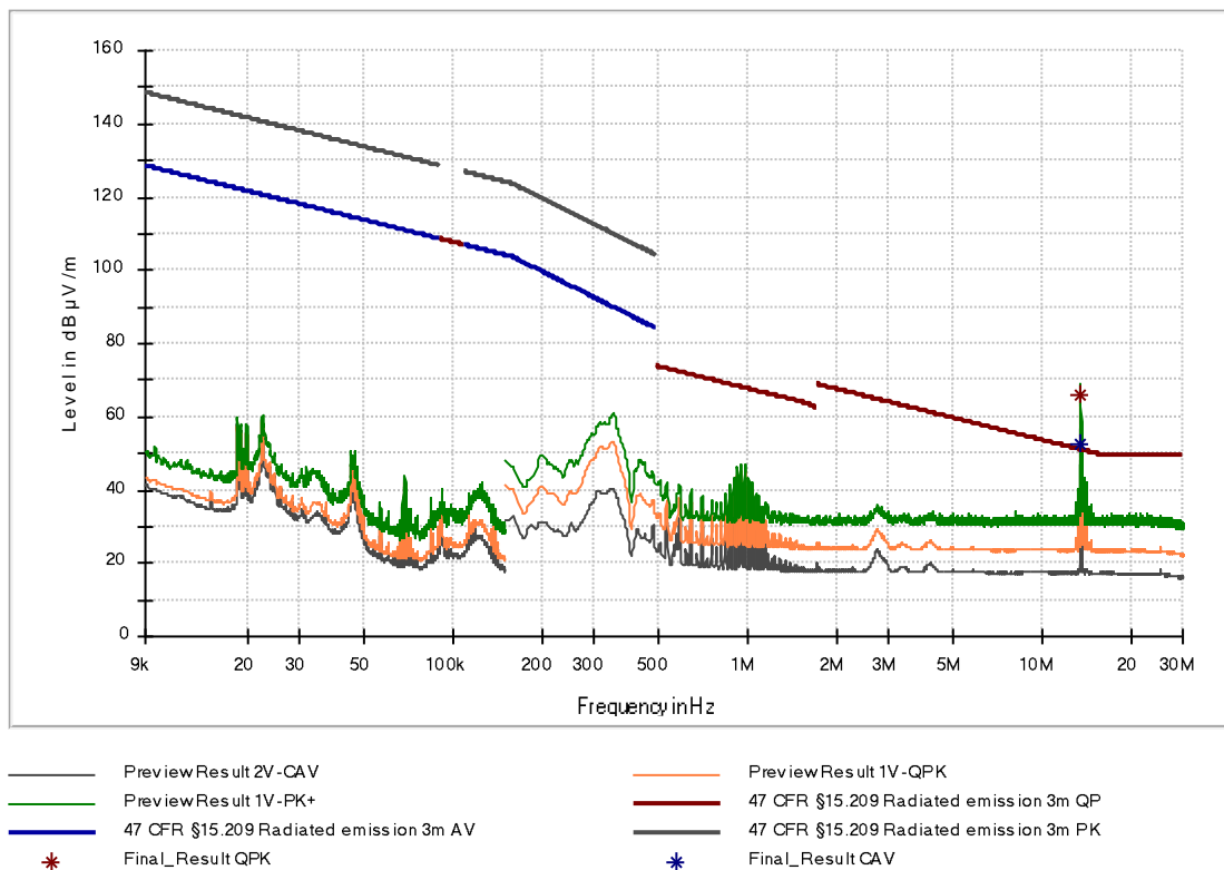
Figure 13: Chart of emissions test below 30 MHz, EUT position Z, without tag, antenna in line at 3 m
