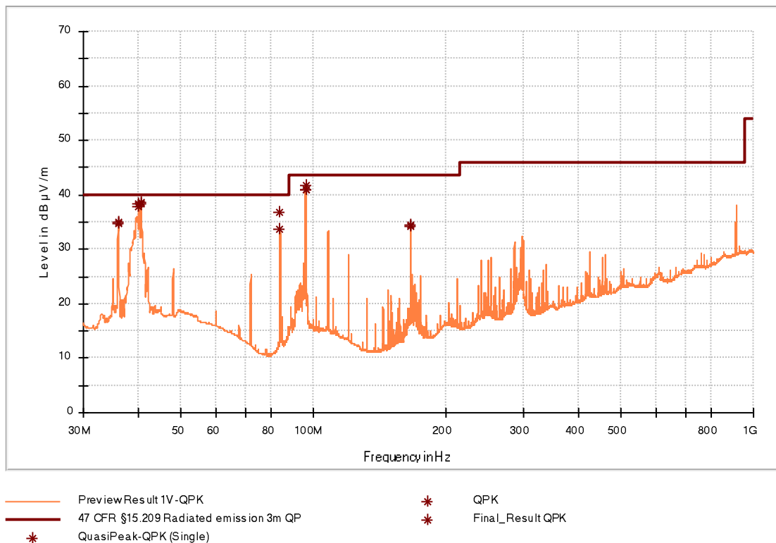
Figure 14: Chart of emissions test from 30 MHz to 1 GHz, EUT position Y, with tag, antenna vertical, at 3 m
