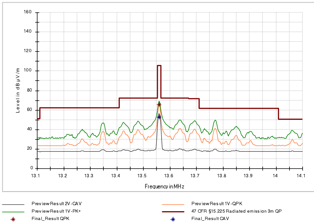
Figure 12: Chart of emission within the band 13.110 MHz to 14.10 MHz, EUT in position Z, without tag, antenna in line at 3 m distance
