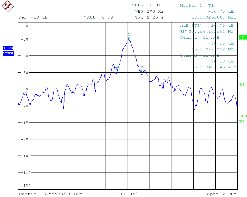
Figure 10: Chart of 20 dB bandwidth tests, with tag
