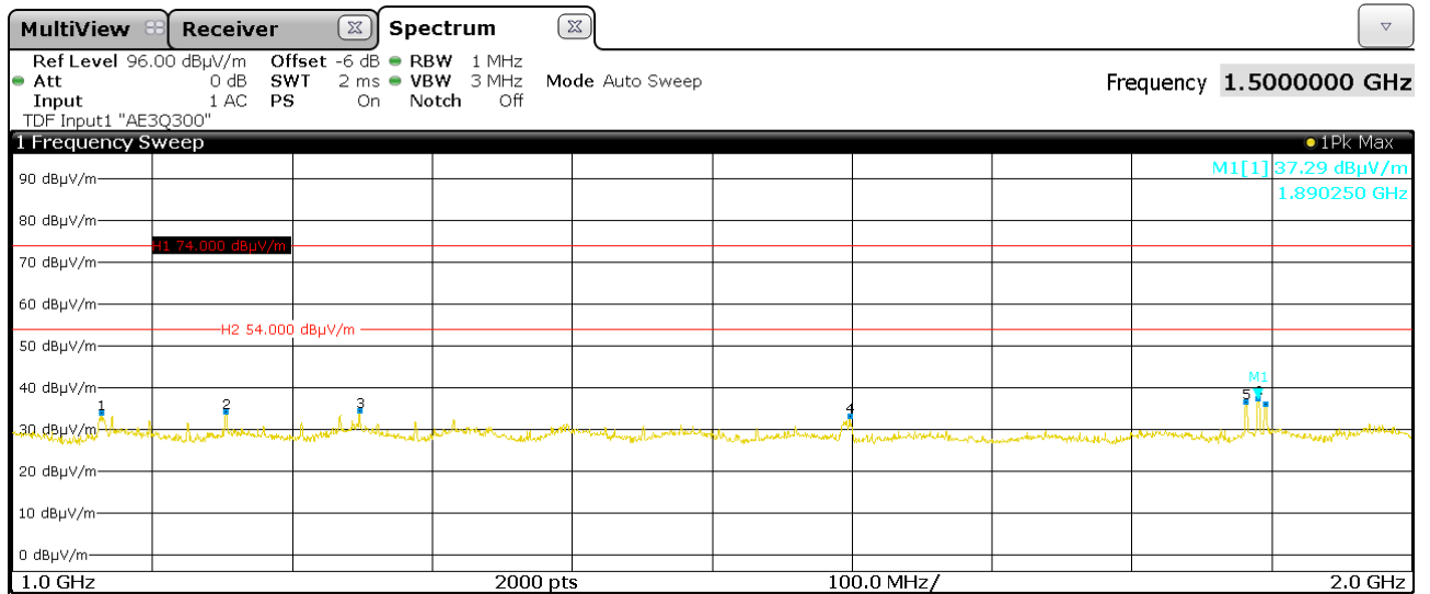
Figure 15: Chart of emissions test from 1 GHz to 2 GHz, EUT position X, with tag, antenna horizontal, at 3 m
