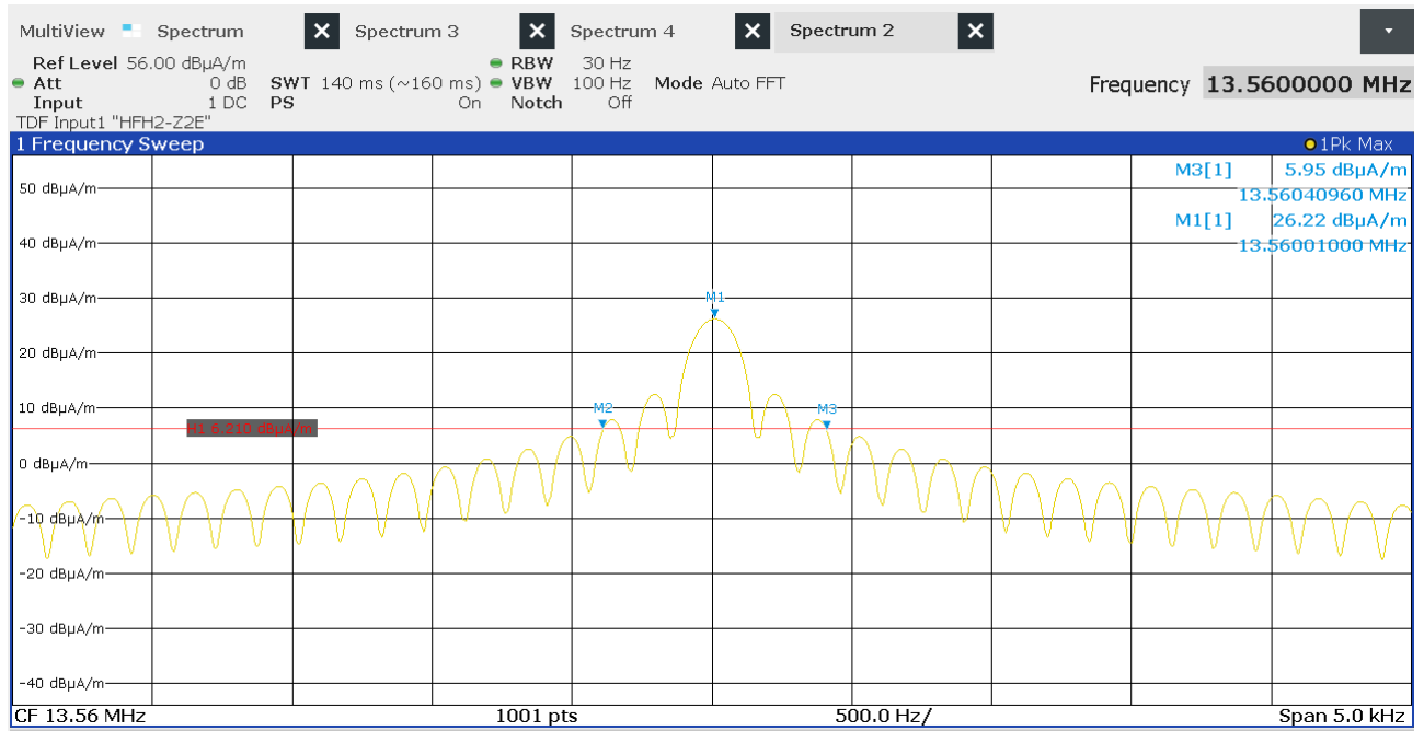
Figure 8: Chart of 20 dB bandwidth tests, without tag
