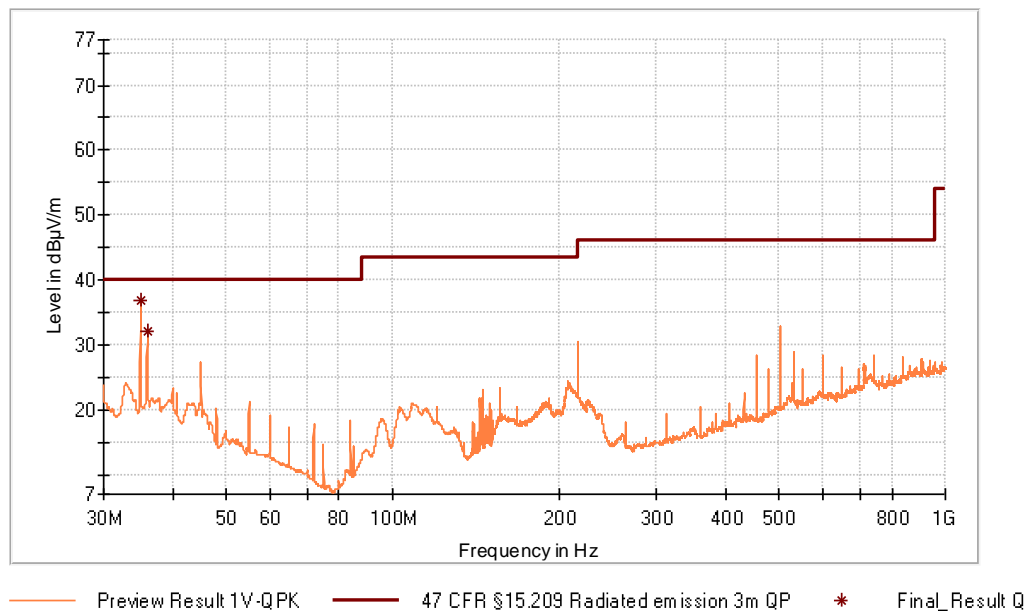
Figure 12: Chart of radiated emissions test from 30 MHz to 1 GHz, EUT position X, antenna vertical, with tag
