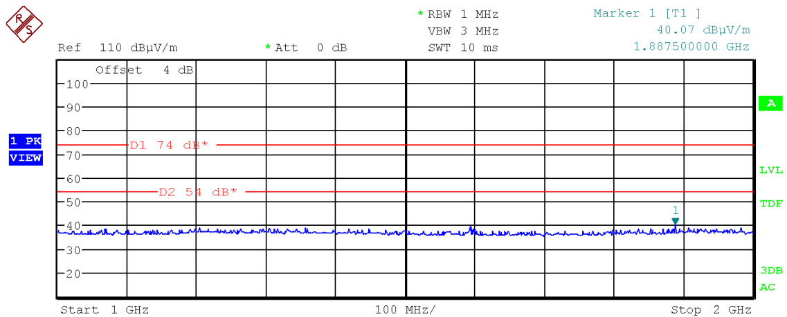
Figure 13: Chart of radiated pre-measurement from 1 GHz to 2 GHz, EUT position Z, with tag, antenna polarization horizontal
