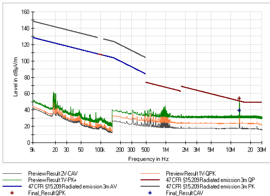
Figure 11: Chart of radiated emissions test below 30 MHz, EUT position Z, antenna in line, without tag
