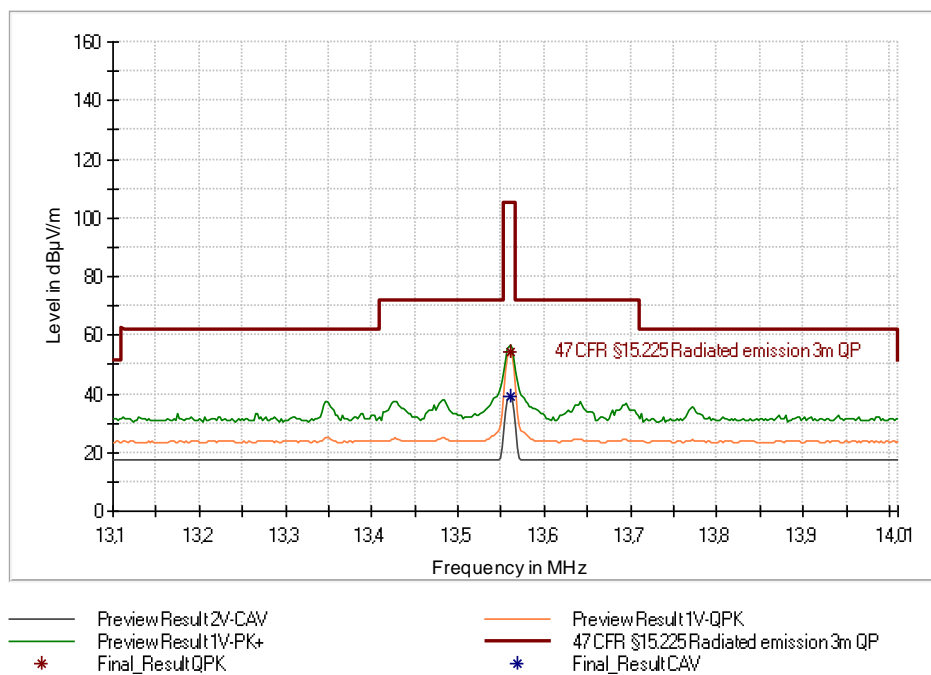
Figure 10: Chart of emission within the band 13.110 MHz to 14.010 MHz, EUT in position Z, without tag, antenna in line at 3 m distance
