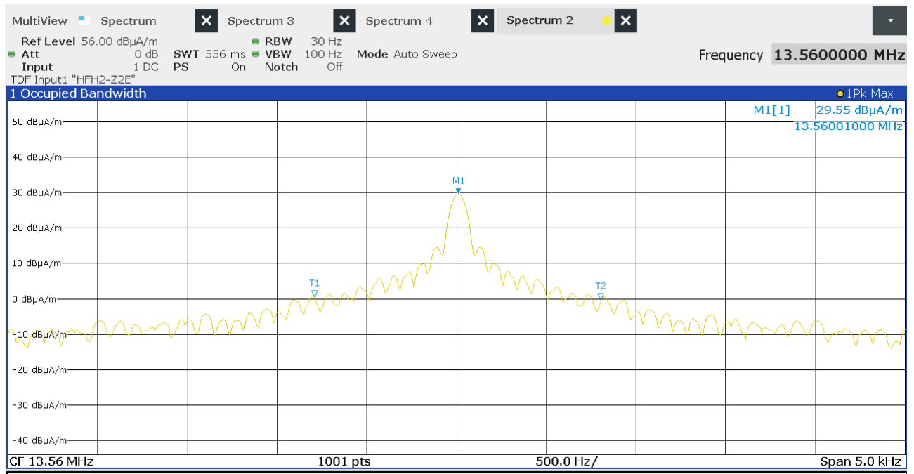
Figure 9: Chart of occupied bandwidth test, without tag
