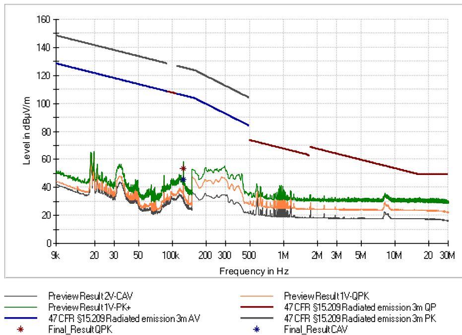
Figure 8: Chart of radiated emissions test below 30 MHz, EUT position Y, with tag, antenna parallel
