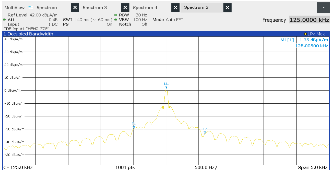
Figure 7: Chart of occupied bandwidth test, without tag
