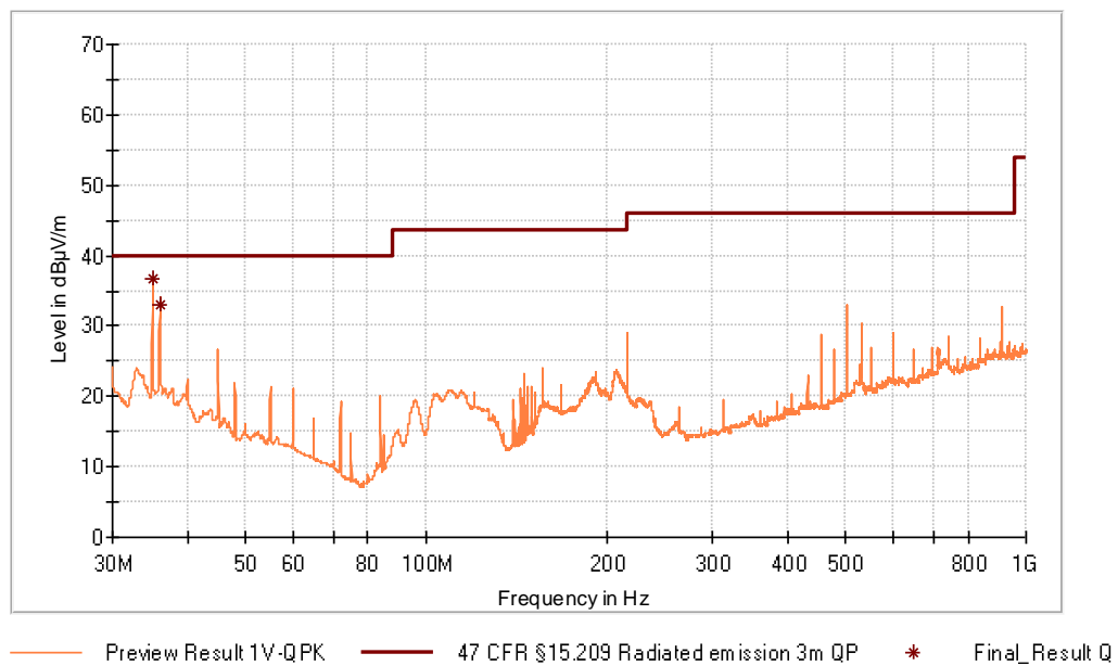
Figure 9: Chart of radiated emissions test from 30 MHz to 1 GHz, EUT position X, with tag, antenna vertical
