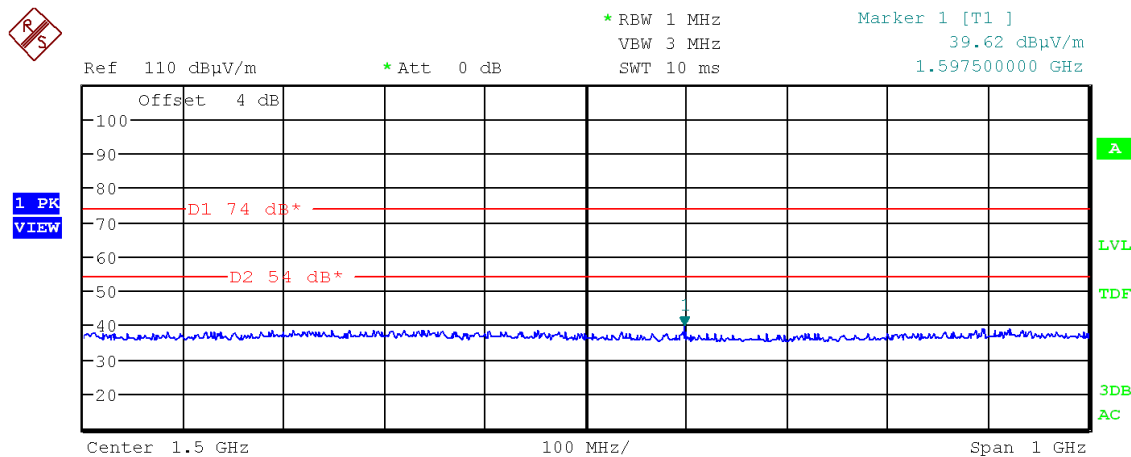
Figure 10: Chart of radiated emissions pre-measurement from 1 GHz to 2 GHz, EUT position Z, with tag, antenna polarization horizontal
