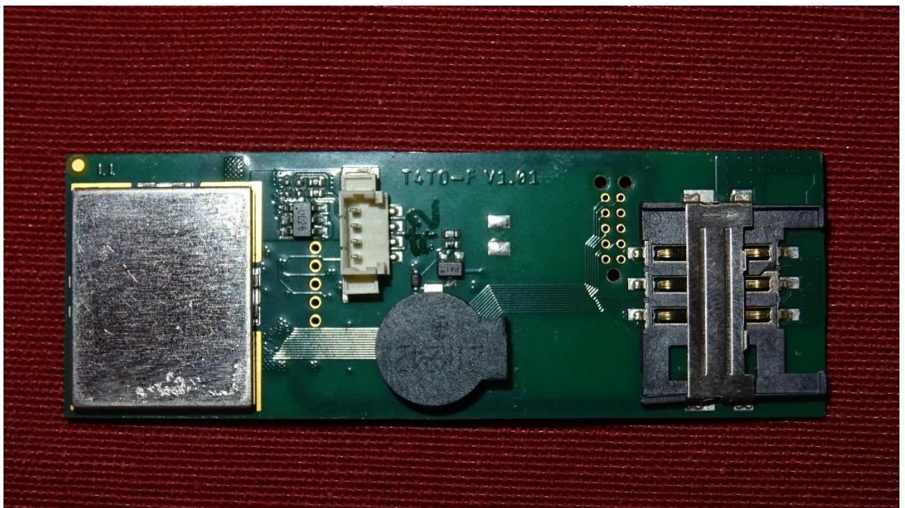
Picture 4: Front view of EUT without SIO card
