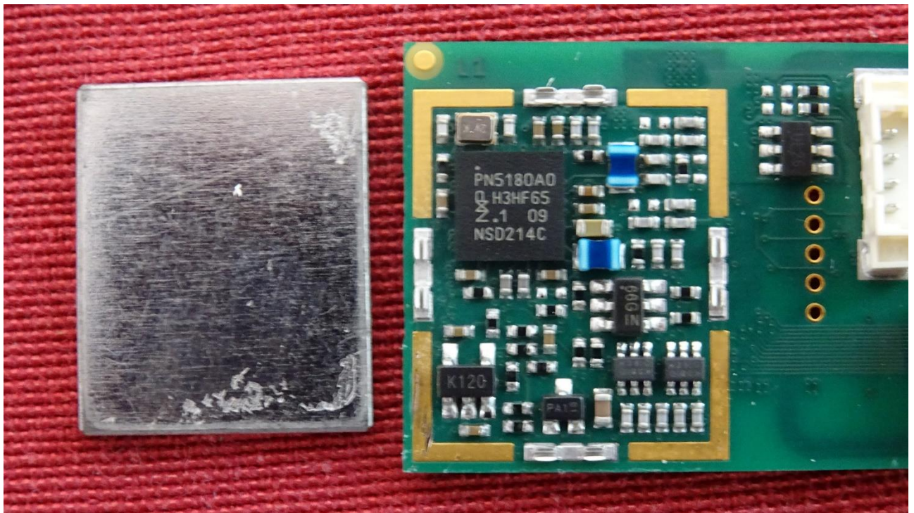
Picture 3: Detailed front view of EUT without shielding
