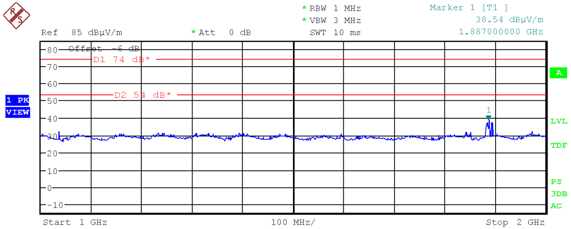
Figure 13: Chart of emissions test from 1 GHz to 2 GHz, EUT position X, with tag, antenna horizontal, at 3 m
