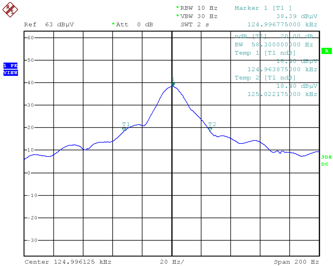
Figure 9: Chart of 20 dB bandwidth tests, without tag
