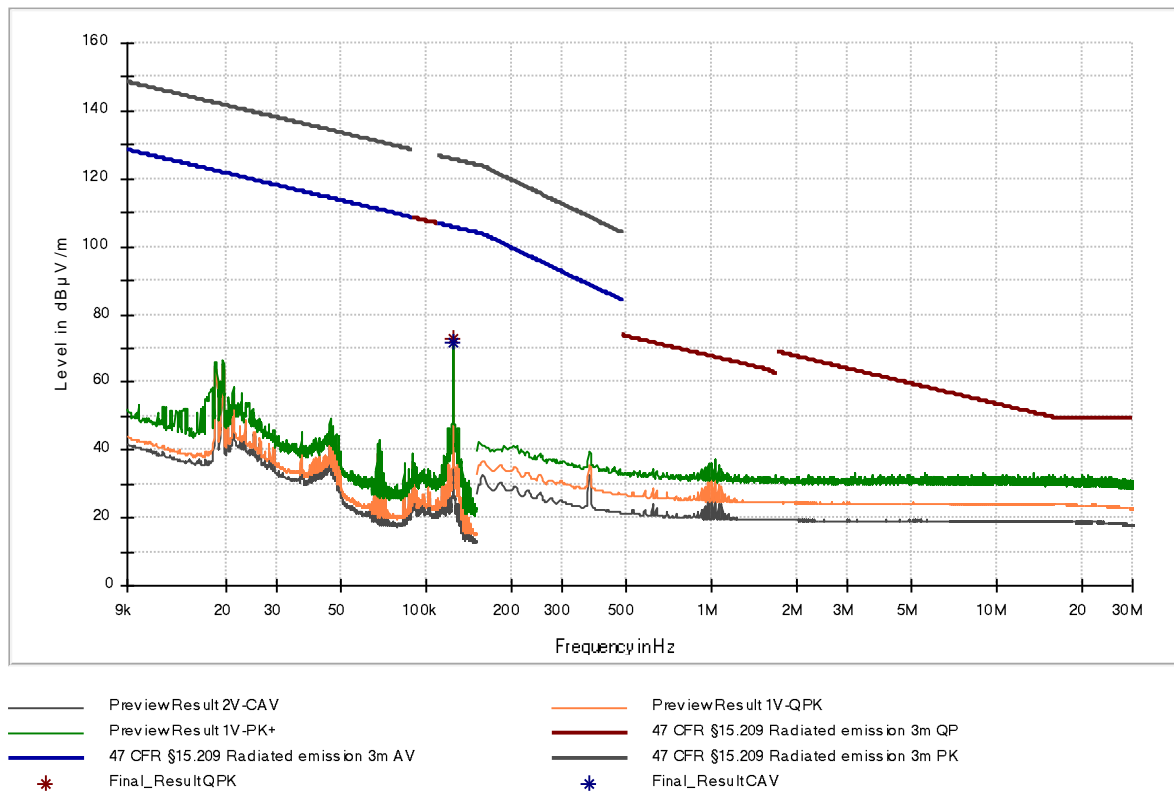
Figure 11: Chart of emissions test below 30 MHz, EUT position Y, without tag, antenna parallel at 3 m
