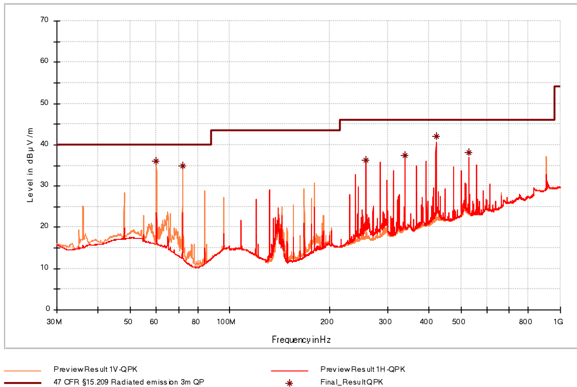
Figure 12: Chart of emissions test from 30 MHz to 1 GHz, EUT position X, with tag, at 3 m
