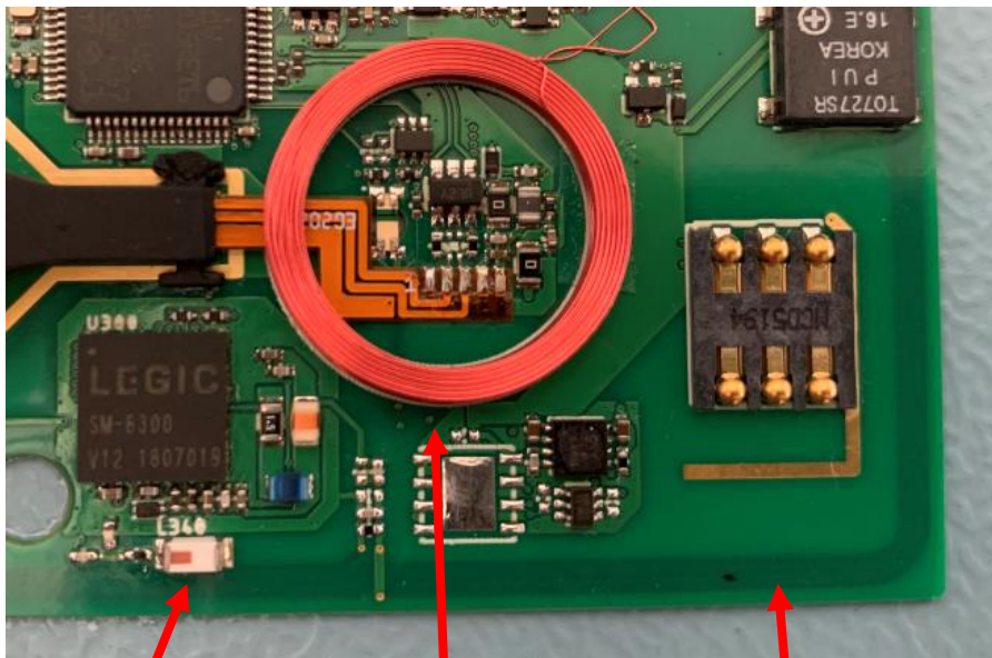
BLE-Antenna (Johanson Technology 2450AT18A100)
