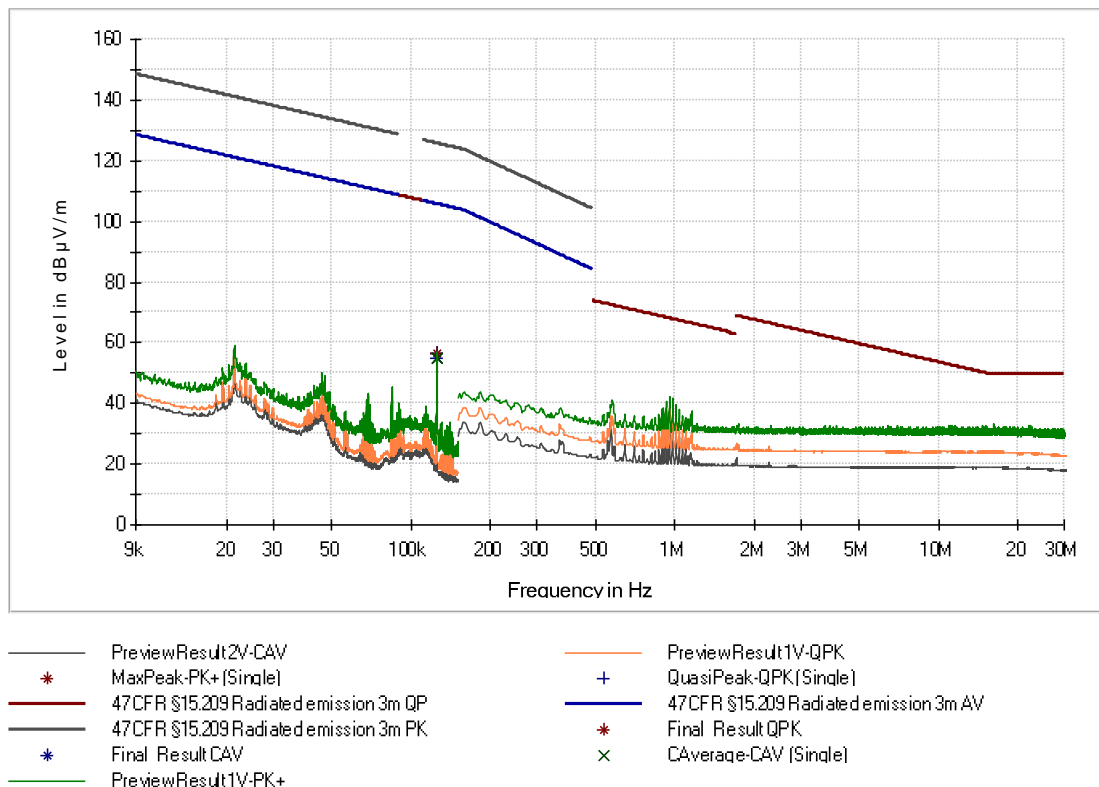
Figure 8: Chart of emissions test below 30 MHz, EUT position Y, without tag, antenna parallel at 3 m
