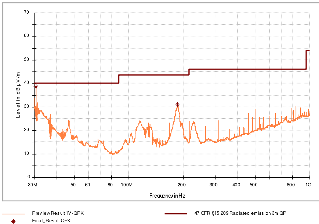
Figure 9: Chart of emissions test from 30 MHz to 1 GHz, EUT position X, with tag, antenna vertical, at 3 m
