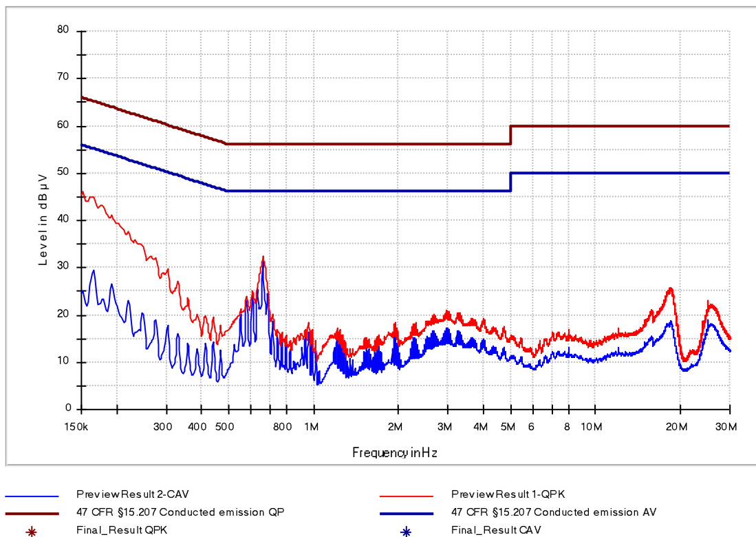
Figure 5: Chart of AC power-line conducted emissions test without termination – phase L1
