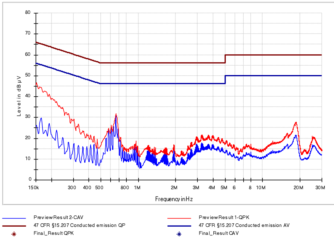
Figure 6: Chart of AC power-line conducted emissions test without termination– phase N
