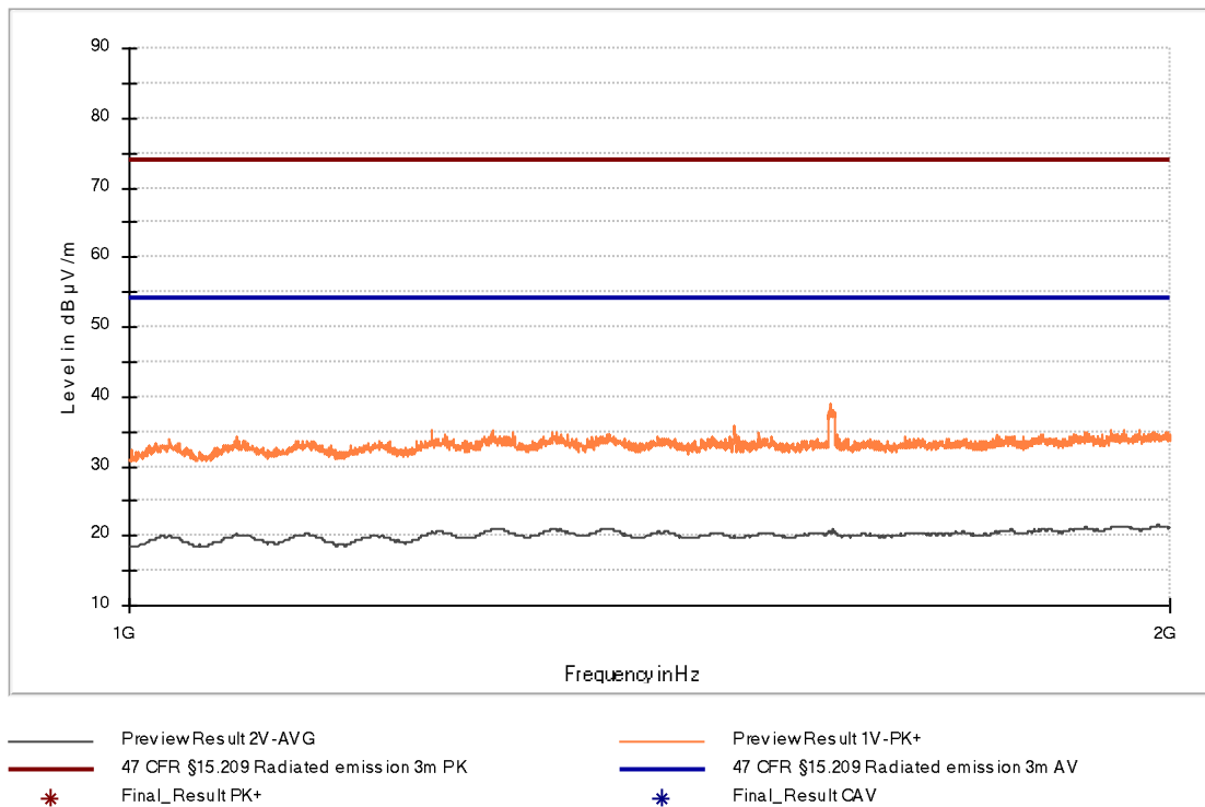
Figure 10: Chart of emissions test from 1 GHz to 2 GHz, EUT position Z, with tag, antenna vertical, at 3 m
