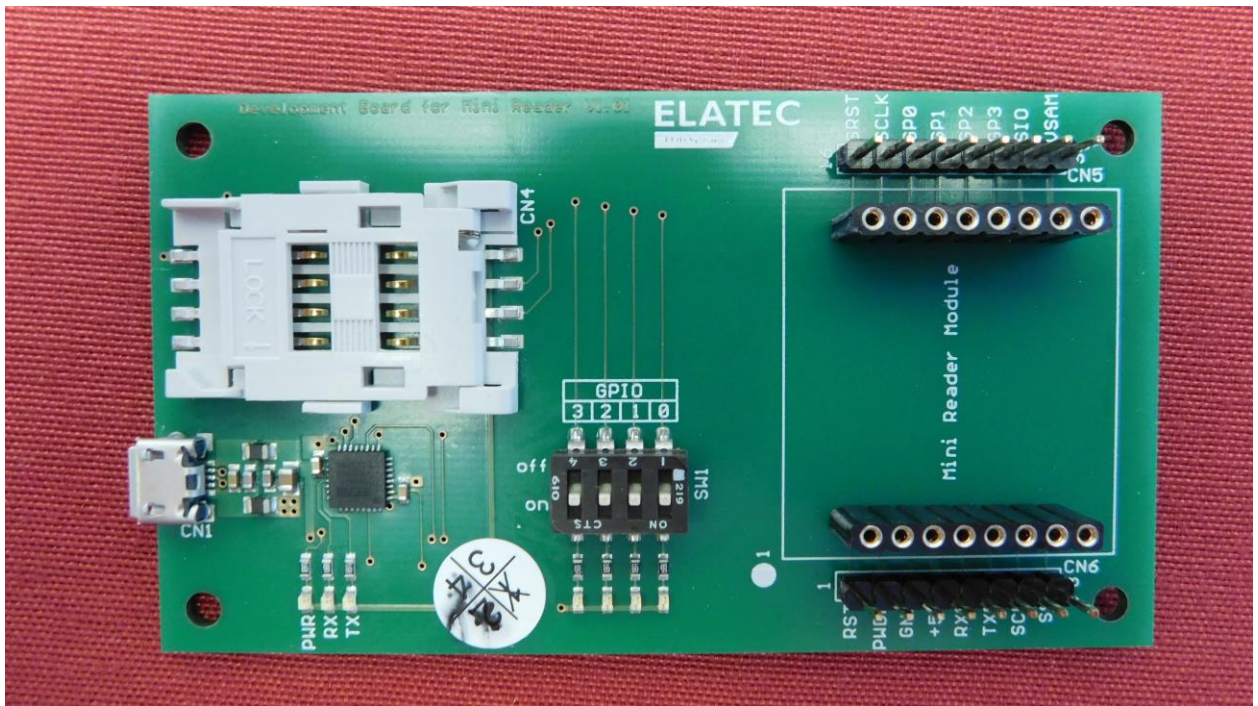
Picture 13: Top view of development board
