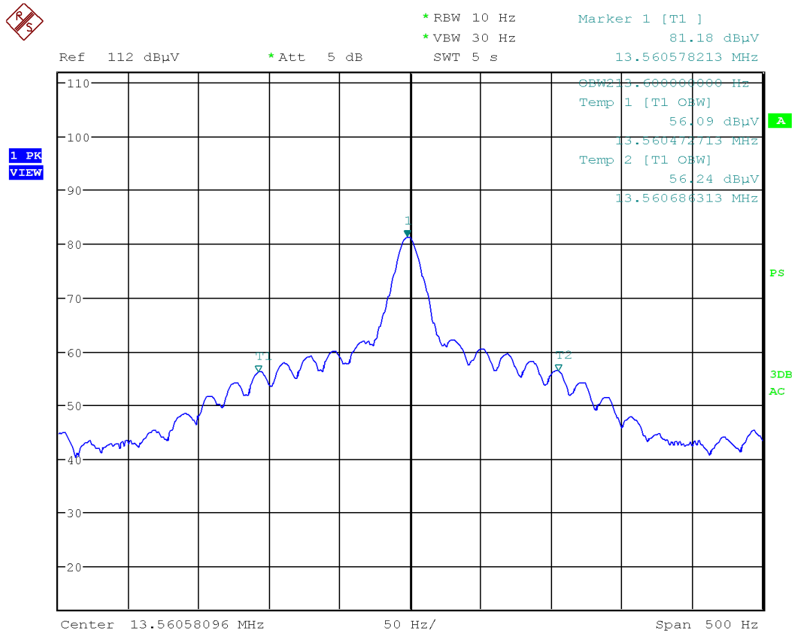
Figure 11: Chart of occupied bandwidth test, with tag
