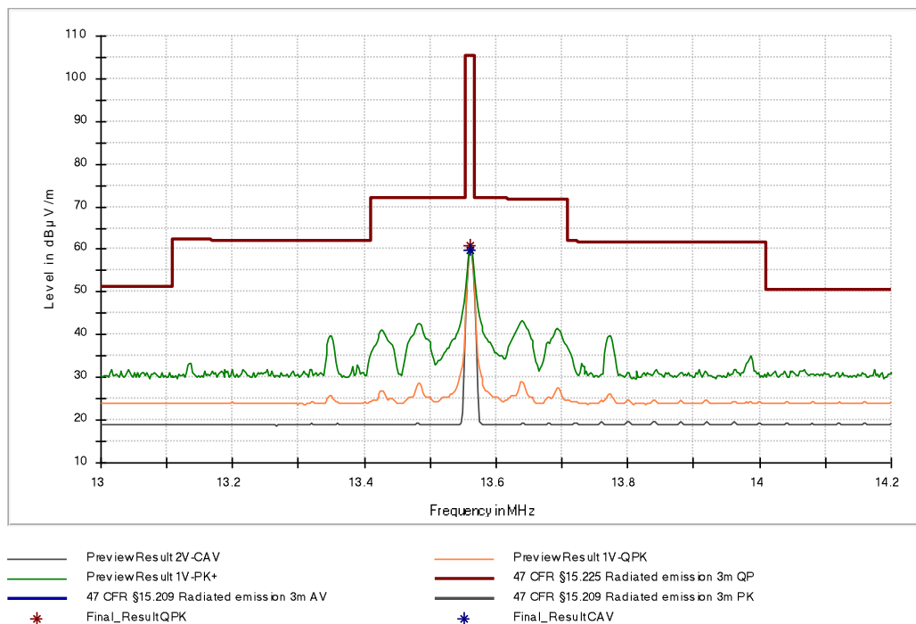
Figure 12: Chart of emission within the band 13.110 MHz to 14.010 MHz, EUT in position Z, without tag, antenna in line, at 3m distance
