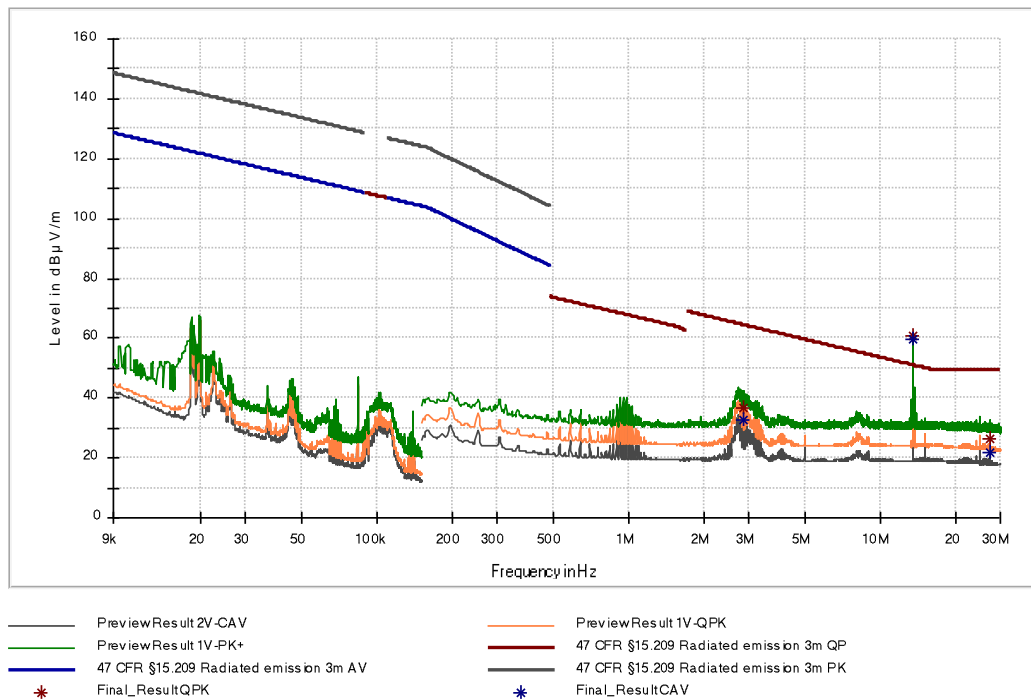
Figure 13: Chart of emissions test below 30 MHz, EUT position X, without tag, antenna in line at 3 m
