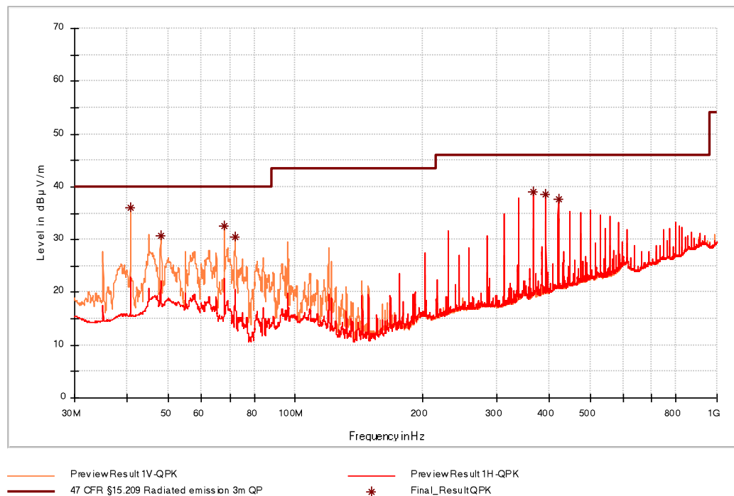
Figure 14: Chart of emissions test from 30 MHz to 1 GHz, EUT position Y, with tag, at 3 m
