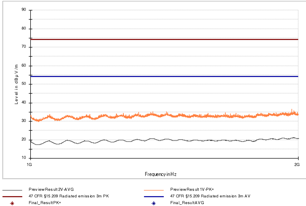
Figure 15: Chart of emissions test from 1 GHz to 2 GHz, EUT position X, with tag, antenna vertical, at 3 m
