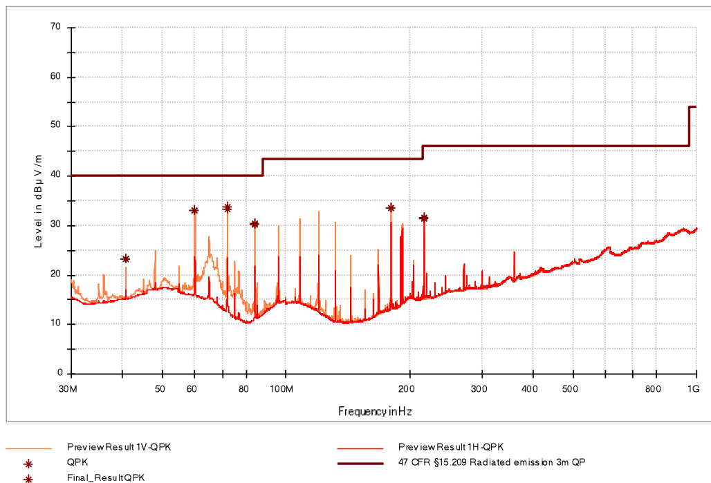
Figure 14: Chart of emissions test from 30 MHz to 1 GHz, EUT position Z, with tag, at 3 m
