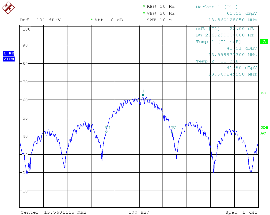
Figure 10: Chart of 20 dB bandwidth tests, without tag
