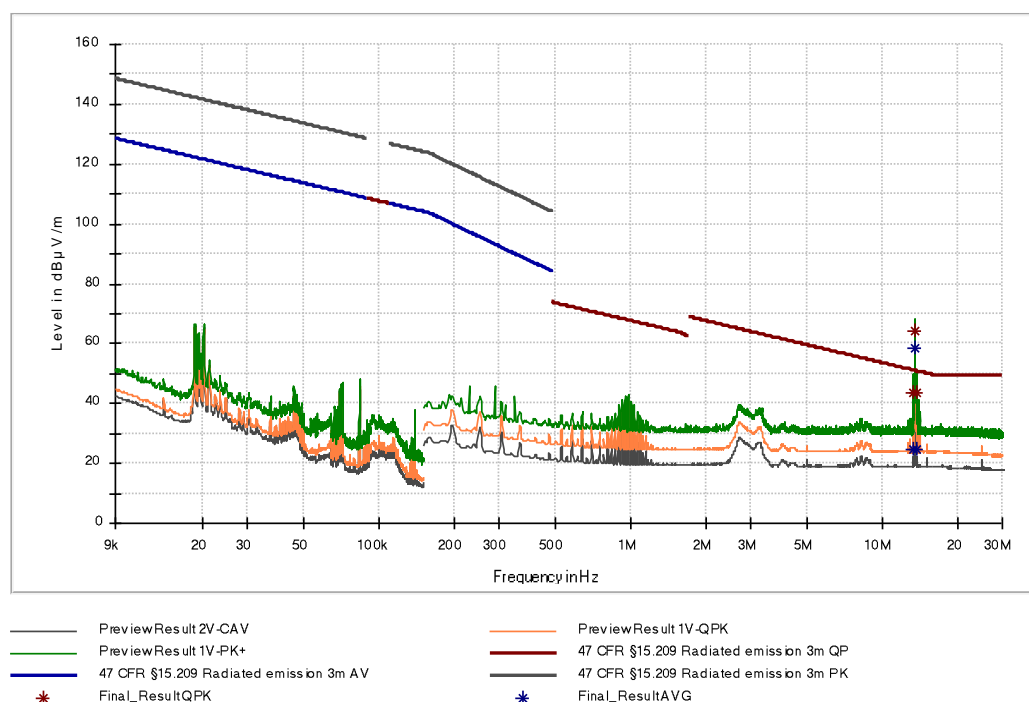
Figure 13: Chart of emissions test below 30 MHz, EUT position Z, with tag, antenna in line at 3 m
