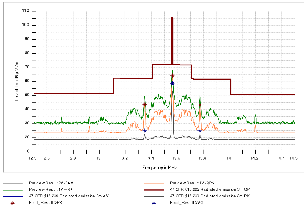
Figure 12: Chart of emission within the band 13.110 MHz to 14.010 MHz, EUT in position Z, with tag, antenna in line, at 3m distance
