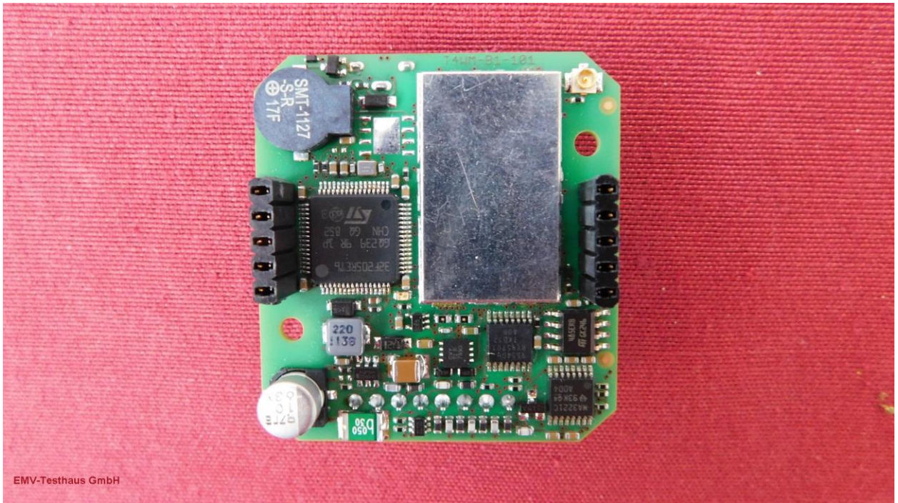
Picture 9: EUT – interface board - top view – with shielding
