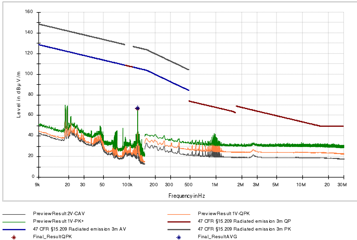
Figure 14: Chart of emissions test below 30 MHz, EUT position X, without tag, antenna parallel at 3 m with active USB interface
