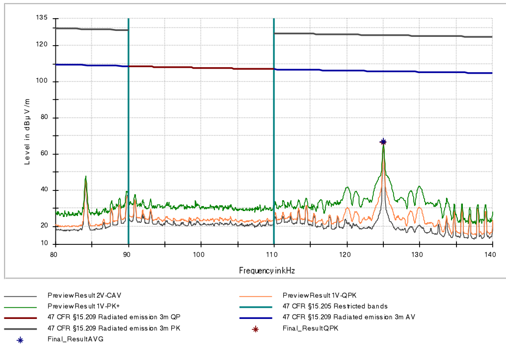
Figure 11: Chart of Restricted Band of Operation
