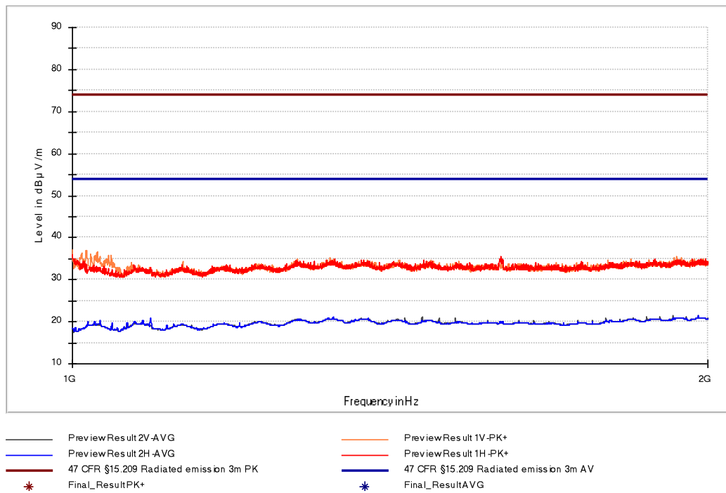
Figure 19: Chart of emissions test from 1 GHz to 2 GHz, EUT position X, with tag, with active RS-232 interface
