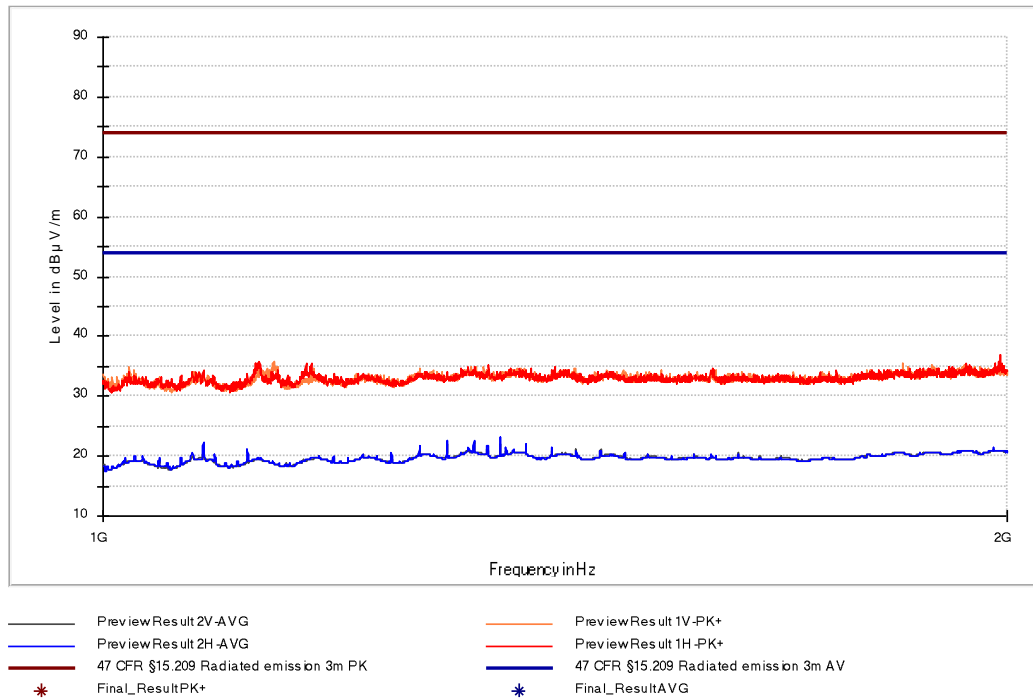
Figure 20: Chart of emissions test from 1 GHz to 2 GHz, EUT position Y, with tag, with active USB interface
