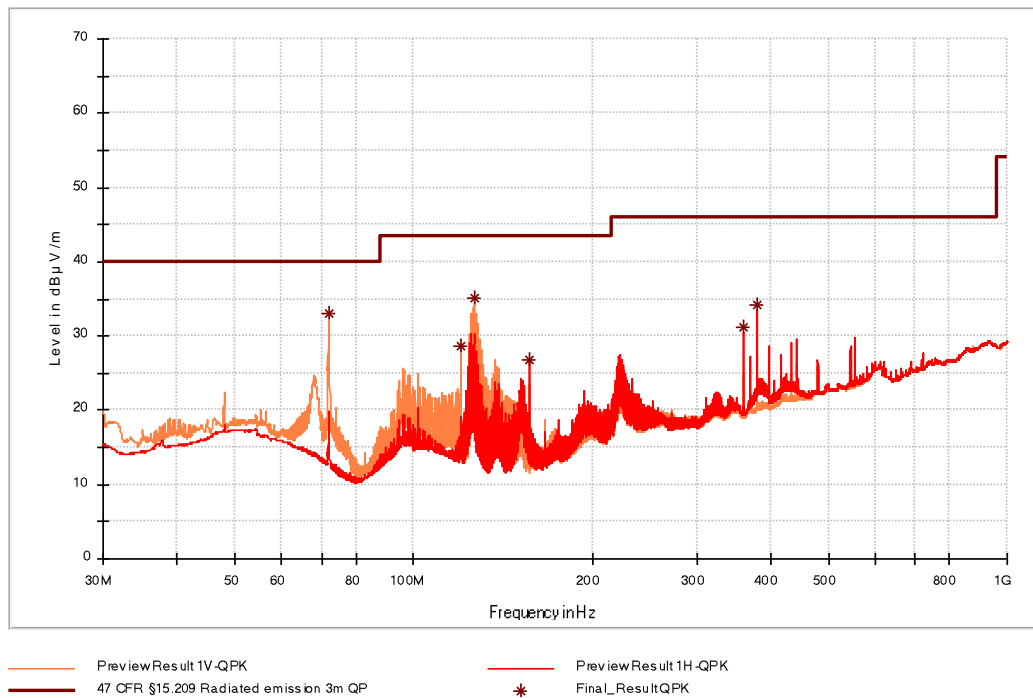
Figure 16: Chart of emissions test from 30 MHz to 1 GHz, EUT position X, with tag at 3 m with active RS-232 interface
