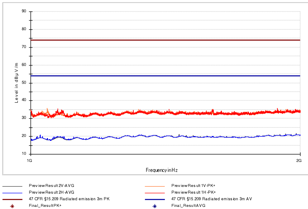
Figure 18: Chart of emissions test from 1 GHz to 2 GHz, EUT position X, with tag, with active RS-485 interface
