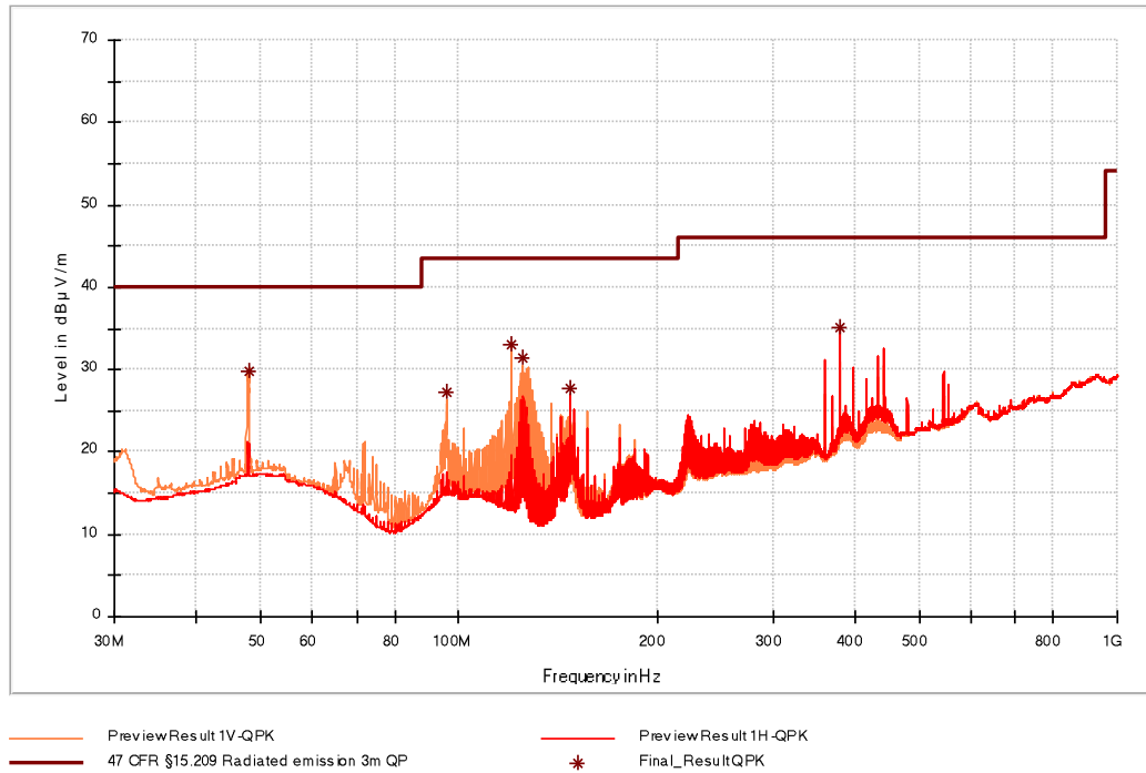
Figure 15: Chart of emissions test from 30 MHz to 1 GHz, EUT position X, with tag at 3 m with active RS-485 interface
