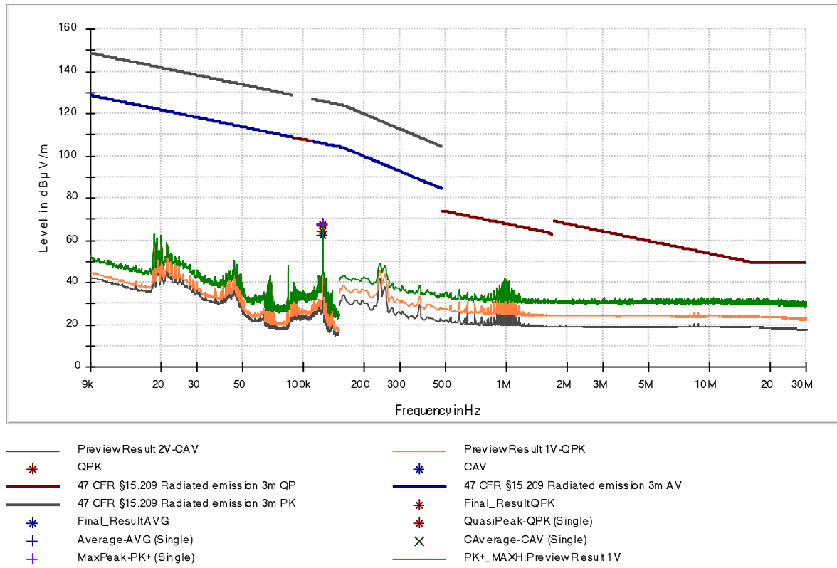
Figure 13: Chart of emissions test below 30 MHz, EUT position Y, without tag, antenna parallel at 3 m with active RS-232 interface
