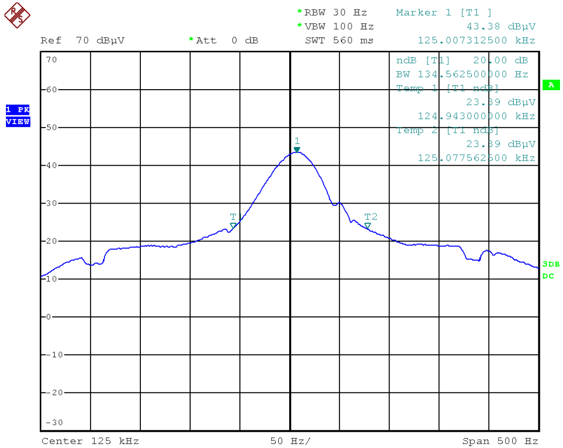
Figure 9: Chart of 20 dB bandwidth test
