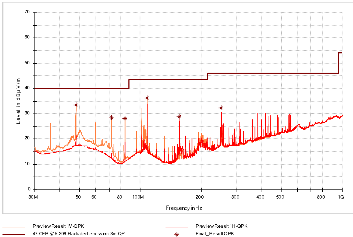
Figure 17: Chart of emissions test from 30 MHz to 1 GHz, EUT position Y, with tag at 3 m with active USB interface
