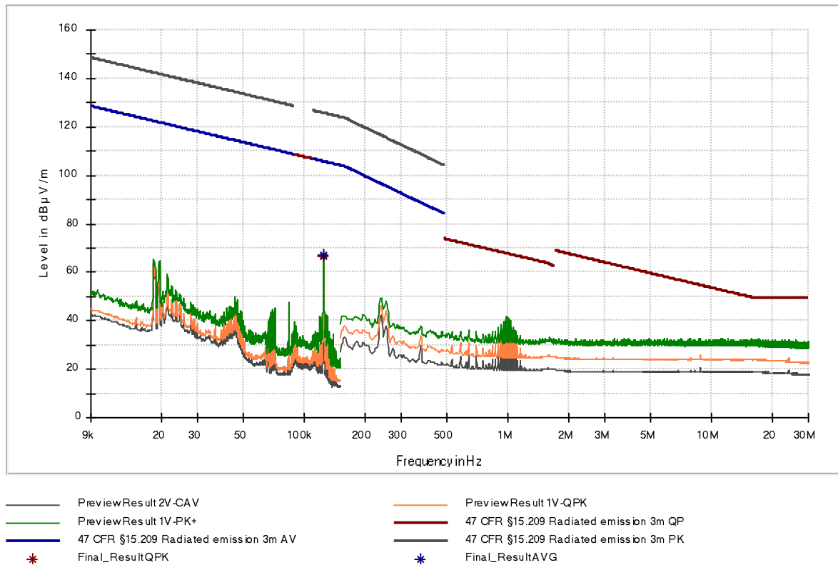
Figure 12: Chart of emissions test below 30 MHz, EUT position X, without tag, antenna parallel at 3 m with active RS-485 interface
