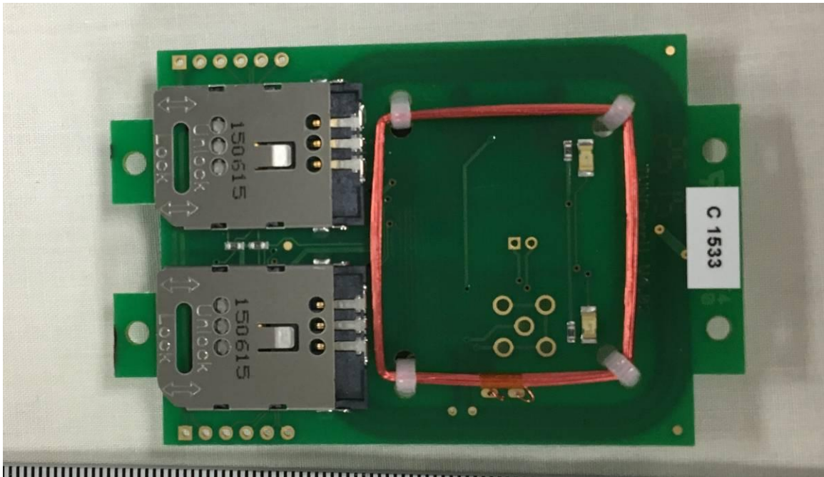
Wire Loop Antenna
