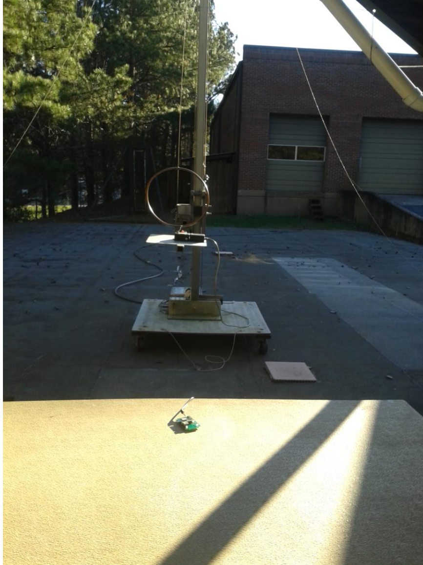
Figure 4. Radiated Emissions Test Setup, Below 30 MHz Testing
