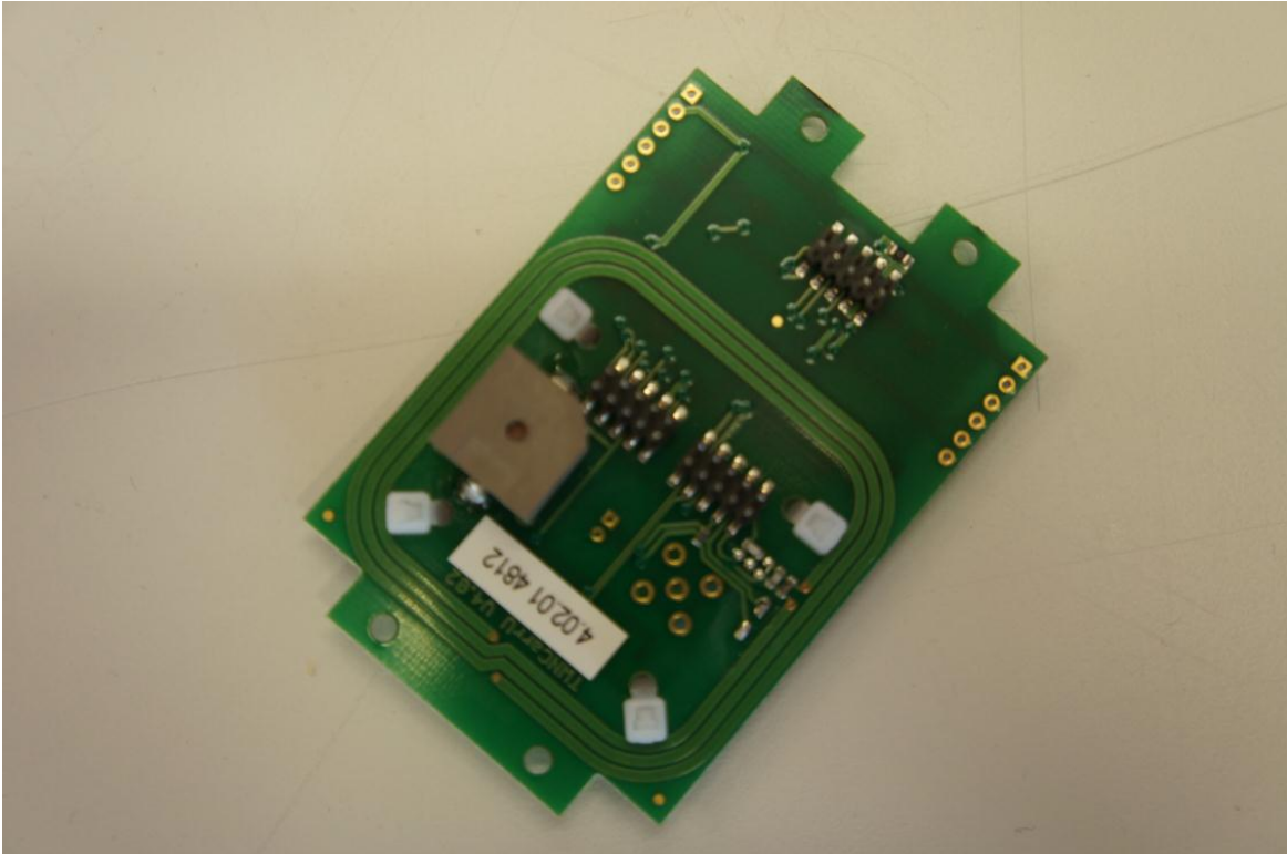
Figure 5. Carrier PCB with Core PCB Removed
