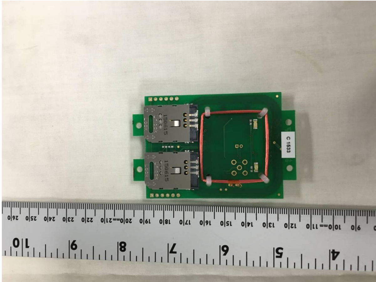
Figure 3. Top of NFC Board/Bare Board Option
