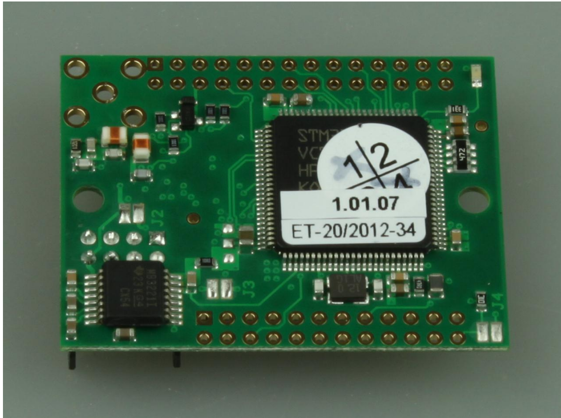
Figure 6. Core PCB Top Side
