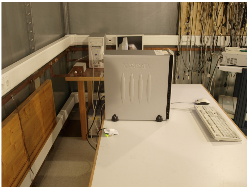
Picture 3: Conducted emission test
