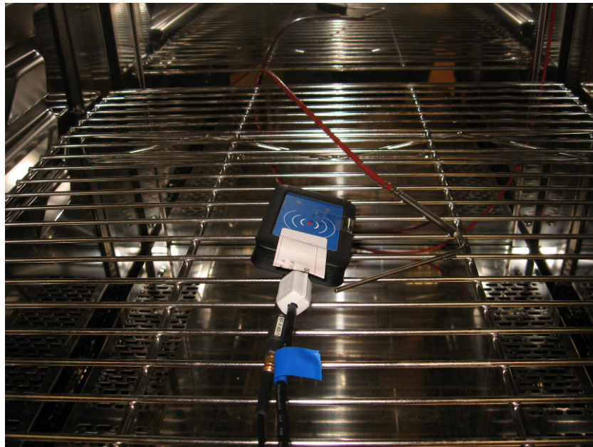
Picture 6: Carrier frequency stability test setup
