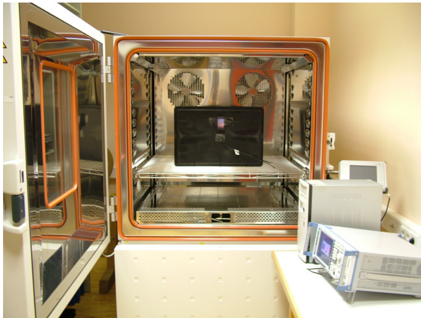
Picture 1-6: Carrier frequency stability test setup
